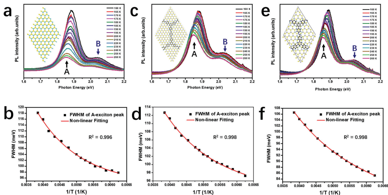
Figure 4. Temperature-dependent PL spectra and plotted FWHM: a,b) \text{MoS}_2 , c,d) \text{MoS}_2 /2D-COF TAPB-PDA heterostructure, and e,f) \text{MoS}_2 /2D-COF TAPB-TFPB heterostructure.
