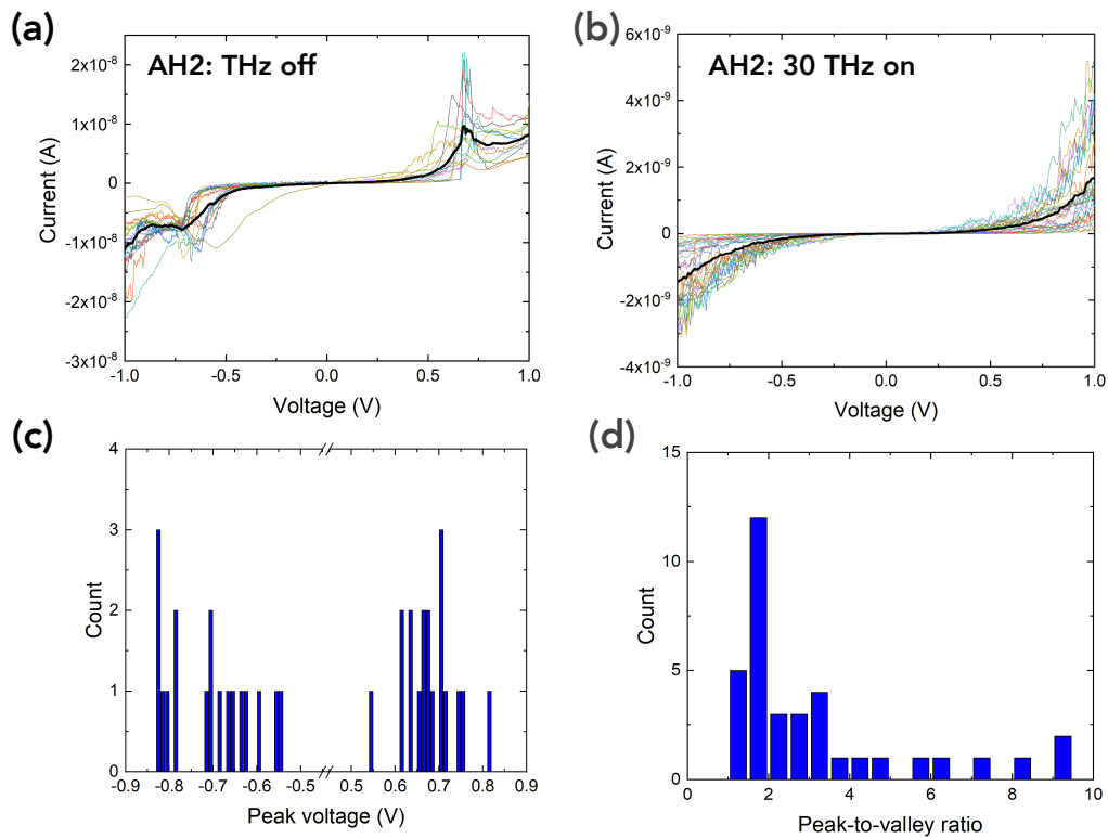
Figure S9. (a) Current-voltage dataset for the ^{75}\text{Au-AH2/PtIr} tip MJJs without THz waves irradiation (18 I-V curves, different colors, acquired at different places on the SAM). The bold black line is the mean \bar{I} -V curve (b) Current-voltage (27 I-V curves, different colors) dataset for the ^{75}\text{Au-AH2/PtIr} tip MJJs under a 30 THz continuous wave irradiation (at a power of 40 mW). The bold black line is the mean \bar{I} -V curve. (c) Histogram of the voltages of the peak currents (from the dataset in panel (a)) for the positive, V_{p+} , and negative, V_{p-} , voltages. (d) Histogram of the peak-to-valley ratios (from the dataset in panel (a)) calculated for every I-V
