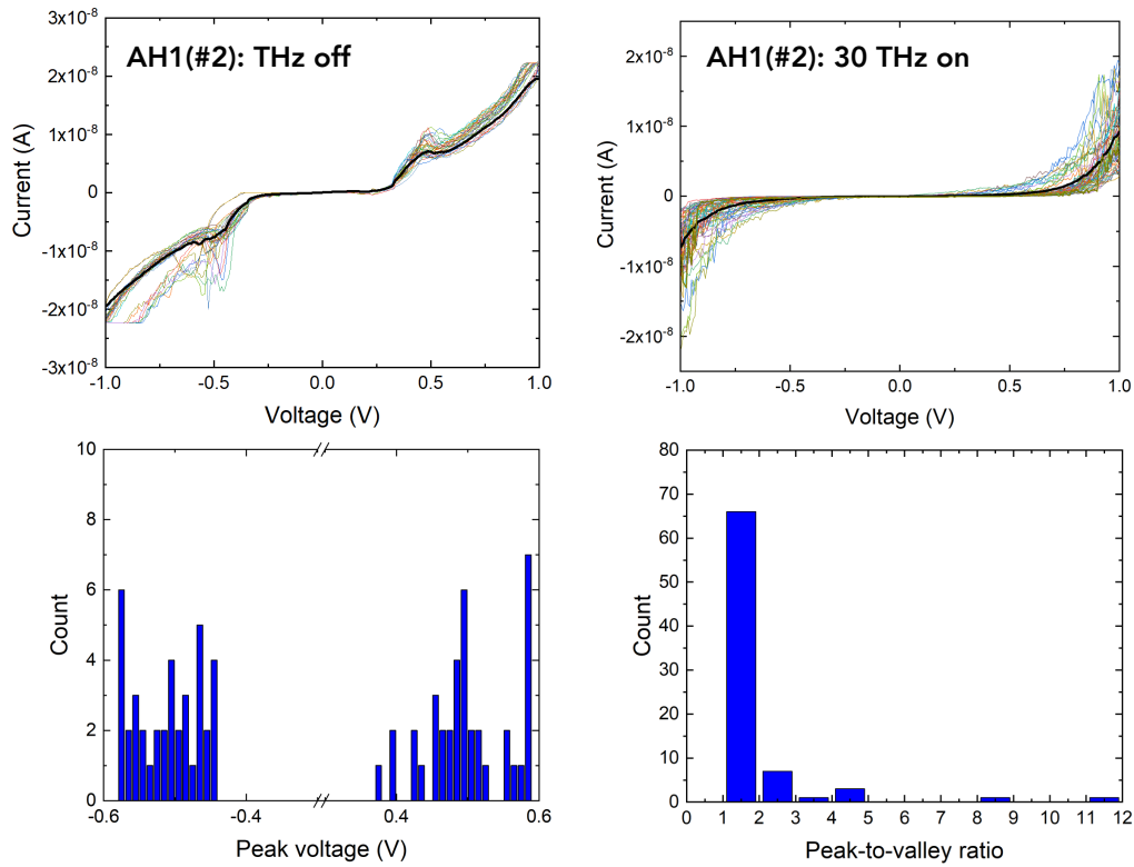
Figure S8. (a) Current-voltage dataset for the ^{TS}\text{Au-AH1}(\#2)//\text{PtIr} tip MJs without THz waves irradiation (39 I-V curves, different colors, acquired at different places on the SAM). The bold black line is the mean \bar{I} -V curve (b) Current-voltage (52 I-V curves, different colors) dataset for the ^{TS}\text{Au-AH1}(\#2)//\text{PtIr} tip MJs under a 30 THz continuous wave irradiation (at a power of 40 mW). The bold black line is the mean \bar{I} -V curve. (c) Histogram of the voltages of the peak currents (from the dataset in panel (a)) for the positive, V_{p+} , and negative, V_{p-} , voltages. (d) Histogram of the peak-to-valley ratios (from the dataset in the panel (a)) calculated as for every I-V.
