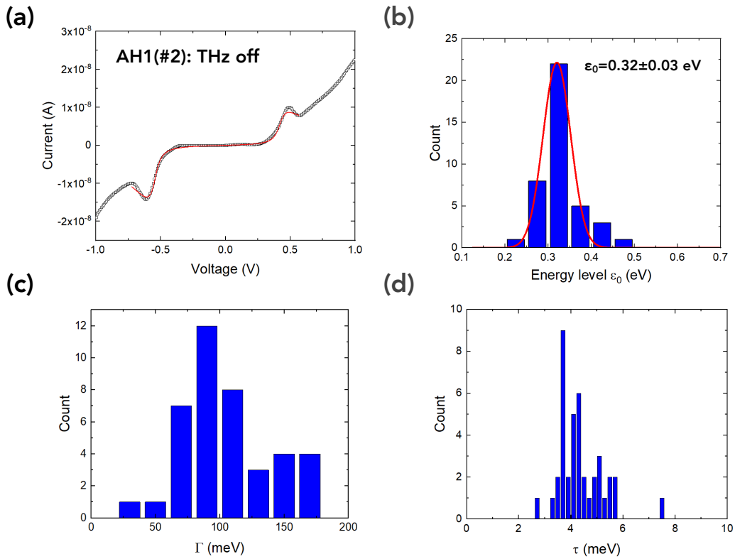
Figure S11. (a) Typical fit of the two-site model on a I-V trace of the ^{75}\text{Au-AH1}(\#2)\text{//PtIr} tip MJ (dataset of Fig. S8a). The fit parameters are: (a) \epsilon_0 = 0.38 eV, \Gamma = 139 meV, \tau = 5.2 meV. The fits are limited between the voltage positions of the
