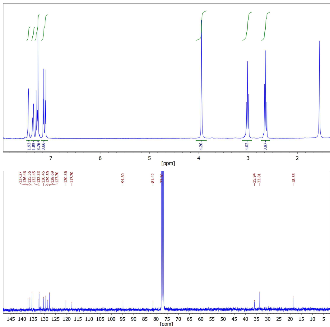
Figure S1. ^1\text{H} (top, 500 MHz) and ^{13}\text{C} (bottom, 125 MHz) NMR spectra of AH1 in \text{CDCl}_3 recorded at 20 °C.
