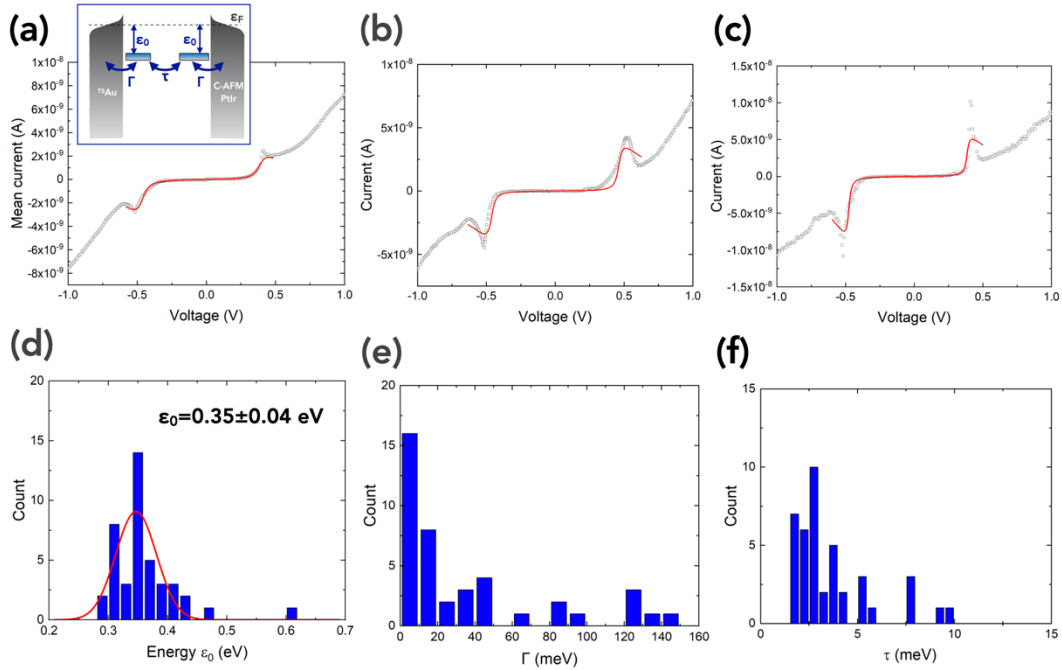
Figure 4. Analysis with a two-site model. Fits of the two-site model on (a) the mean \bar{I} -V of the ^{TS}\text{Au} -AH1//PtIr tip MJ (dataset of Fig. 2a) and (b-c) two typical I-V from the dataset with a marked NDC behavior. The fit parameters are: (a) \epsilon_0=0.32 eV, \Gamma=101 meV, \tau=2 meV; (b) \epsilon_0=0.35 eV, \Gamma=35 meV, \tau=4 meV; (c) \epsilon_0=0.33 eV, \Gamma=119 meV, \tau=3.5 meV. The fits are limited between the voltage positions of the two current valleys since the monotonous increase of the background “off-resonance” current with the voltage at higher voltages is not taken into account by this model (see Methods). (d-f) Histograms of the fit parameters obtained by fitting all individual I-V curves of the dataset (Fig. 2a): (d) energy of molecular orbital \epsilon_0 , the red line is the fit with a Gaussian distribution; (e) electrode coupling energy \Gamma and (f) intramolecular electronic coupling energy \tau .
