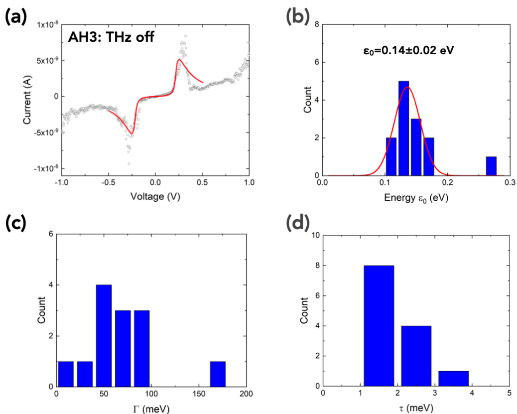
Figure S12. (a) Typical fit of the two-site model on a I-V trace of the ^{TS}\text{Au-AH3//PtIr} tip MJ (dataset of Fig. S7a). The fit parameters are: (a) \epsilon_0 = 0.16 eV, \Gamma = 29 meV, \tau = 2.7 meV. The fits are limited between the voltage positions of the two current valleys since the monotonous increase of the background “off-resonance” current with the voltage at higher voltages is not taken into account by this model (see Methods). (b-d) Histograms of the fit parameters obtained by fitting all individual I-V curves of the dataset (Fig. S8-a): (b) energy of molecular orbital \epsilon_0 , the red line is the fit with a Gaussian distribution; (c) electrode coupling energy \Gamma and (d) intramolecular electronic coupling energy \tau .
