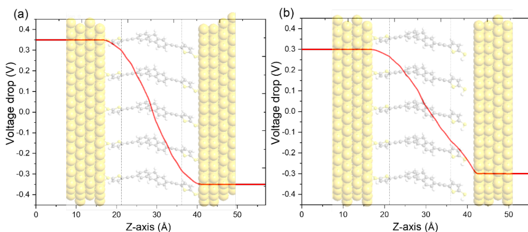
Figure S14. The calculated total voltage drop across the device projected on molecular axis (Z axis) in (a) the Au-AH1-Au junction under 0.7V and in (b) the Au-AH1//Au junction under 0.6V ( i.e. at peak voltage). A voltage of 0.58 V (0.41 V) is
