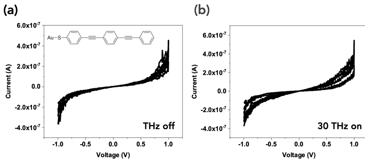
Extended data Fig. 2. Control experiments on OPE MJ. Current-voltage curves (10 traces) measured for a ^{75}\text{Au} -OPE3//PtIr tip: (a) without THz irradiations, (b) under 30 THz irradiation at P=40 mW.
