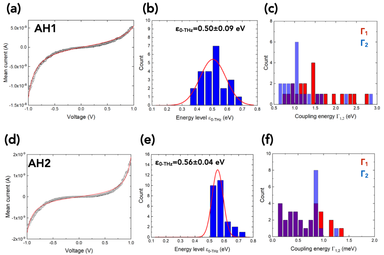
Extended data Fig. 4. Single energy level model. (a) Fit of the SEL model (red line) on the mean \bar{I} -V curve (AH1 junction, from Fig. 2b) with the parameters: \epsilon_{0-THz}=0.47 eV, \Gamma_1=2.0 meV and \Gamma_2=1.7 meV. (b) Histograms of the \epsilon_{0-THz} values from the fit of all individual I-V traces in the dataset of Fig. 2b. The histogram is fitted by a gaussian distribution with \epsilon_{0-THz}=0.50\pm 0.09 eV. (c) Histograms of the fitted electrode coupling energies. \Gamma_1 and \Gamma_2 span in the range \approx 0.5 to 3 meV. (d) Fit of the SEL model (red line) on the mean \bar{I} -V curve (AH2 junction, from extended data Fig. 1) with the parameters: \epsilon_{0-THz}=0.56 eV, \Gamma_1=0.59 meV and \Gamma_2=0.61 meV. (e) Histograms of the \epsilon_{0-THz} values from the fit of all individual I-V traces in the dataset of Fig. 2b. The histogram is fitted by a gaussian distribution with \epsilon_{0-THz}=0.56\pm 0.04 eV. (f) Histograms of the fitted electrode coupling energies. \Gamma_1 and \Gamma_2 span in the range \approx 0.1 to 1.5 meV.
