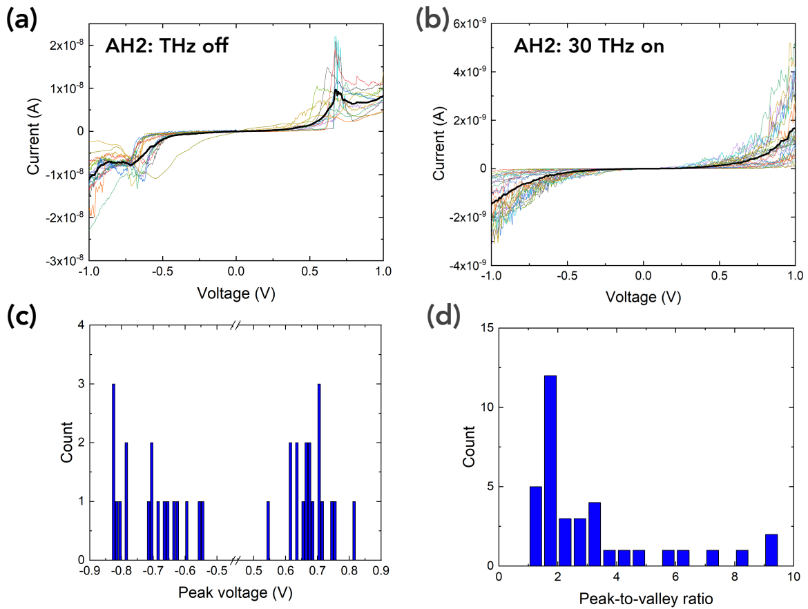
Extended data Fig. 1. NDC and THz switching effects of the AH2 MJs. (a) Current-voltage dataset for the ^{75}\text{Au-AH2//PtIr} tip MJs without THz waves irradiation (39 I-V curves, different colors, acquired at different places on the SAM, see Methods). The bold black line is the mean \bar{I} -V curve (b) Current-voltage (27 I-V curves, different colors) dataset for the ^{75}\text{Au-AH2//PtIr} tip MJs under a 30 THz continuous wave irradiation (at a power of 40 mW). The bold black line is the mean \bar{I} -V curve. (c) Histogram of the voltages of the peak currents (from the dataset in panel (a)) for the positive, V_{p+} , and negative, V_{p-} , voltages. (d) Histogram of the peak-to-valley ratios (from the dataset in panel (a)) calculated for every I-V.
