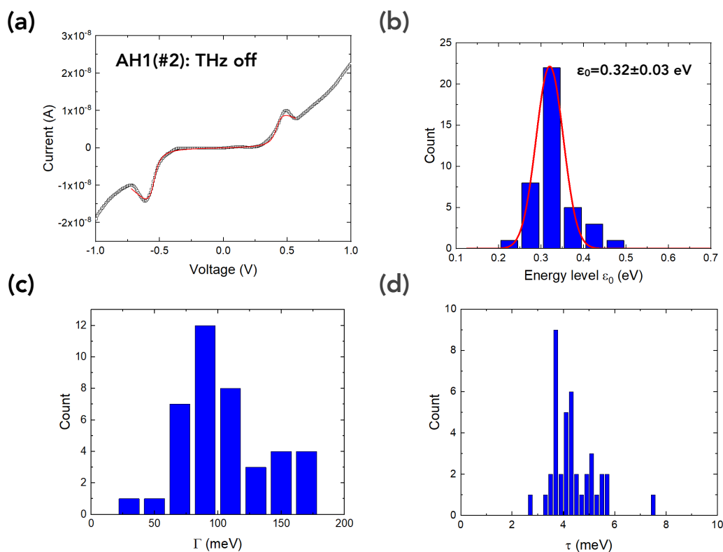
Figure S9. (a) Typical fit of the two-site model on a I-V trace of the ^{75}\text{Au} -AH1(#2)//PtIr tip MJ (dataset of Fig. S7a). The fit parameters are: (a) \epsilon_0 = 0.38 eV, \Gamma = 139 meV, \tau = 5.2 meV. The fits are limited between the voltage positions of the two current valleys since the monotonous increase of the background “off-resonance” current with the voltage at higher voltages is not taken into account by this model (see Methods). (b-d) Histograms of the fit parameters obtained by fitting all individual I-V curves of the dataset (Fig. S8-a): (b) energy of molecular orbital \epsilon_0 , the red line is the fit with a Gaussian distribution; (c) electrode coupling energy \Gamma and (d) intramolecular electronic coupling energy \tau .
