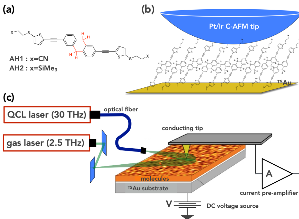
Figure 1. Illustration of the molecular junctions and experiments. (a) Chemical structure of the 3,3'-(((9,10-dihydroanthracene-2,6-diyl)bis(ethyne-2,1-diyl))bis(thiophene-5,2-diyl))bis(sulfanediyl)dipropanenitrile ( AH1 ) and 2,6-bis((5-((2-(trimethylsilyl)ethyl)thio)thiophen-2-yl)ethynyl)-9,10-dihydroanthracene ( AH2 ). (b) Scheme of the molecular junction with the SAM connected by the tip of the C-AFM. (c) Scheme of the experiment. THz waves are focalized under the tip of the C-AFM (see details in Methods).
