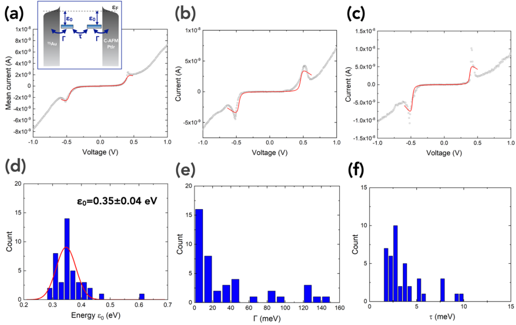
Figure 4. Analysis with a two-site model. Fits of the two-site model on (a) the mean \bar{I} - V of the ^{TS}\text{Au} -AH1//PtIr tip MJ (dataset of Fig. 2a) and (b-c) two typical I - V from the dataset with a marked NDC behavior. The fit parameters are: (a) \epsilon_0=0.32 eV, \Gamma=101 meV, \tau=2 meV; (b) \epsilon_0=0.35 eV, \Gamma=35 meV, \tau=4 meV; (c) \epsilon_0=0.33 eV, \Gamma=119 meV, \tau=3.5 meV. The fits are limited between the voltage positions of the two current valleys since the monotonous increase of the background “off-resonance” current with the voltage at higher voltages is not taken into account by this model (see Methods). (d-f) Histograms of the fit parameters obtained by fitting all individual I - V curves of the dataset (Fig. 2a): (d) energy of molecular orbital \epsilon_0 , the red line is the fit with a Gaussian distribution; (e) electrode coupling energy \Gamma and (f) intramolecular electronic coupling energy \tau .
