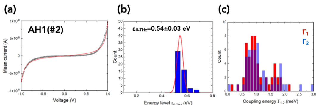
Figure S10. (a) Fit of the SEL model (red line) on the mean \bar{I} -V curve (AH1(#2) junction, from Fig. S8b) with the parameters: \epsilon_{0-THz}=0.53 eV, \Gamma_1=0.9 meV and \Gamma_2=1.0 meV. (b) Histograms of the \epsilon_{0-THz} values from the fit of all individual I-V traces in the dataset of Fig. S8b. The histogram is fitted by a gaussian distribution with \epsilon_{0-THz}=0.54 \pm 0.03 eV. (c) Histograms of the fitted electrode coupling energies. \Gamma_1 and \Gamma_2 span in the range \approx 0.5 to 3 meV.
