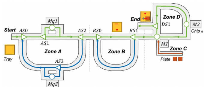
Fig. 2. The TRACILOGIS platform layout [14]
