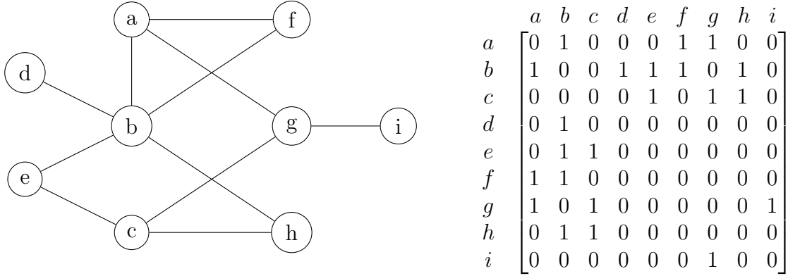
Figure 2: A graph and its adjacency matrix
