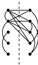
Figure 1: An example of a split
