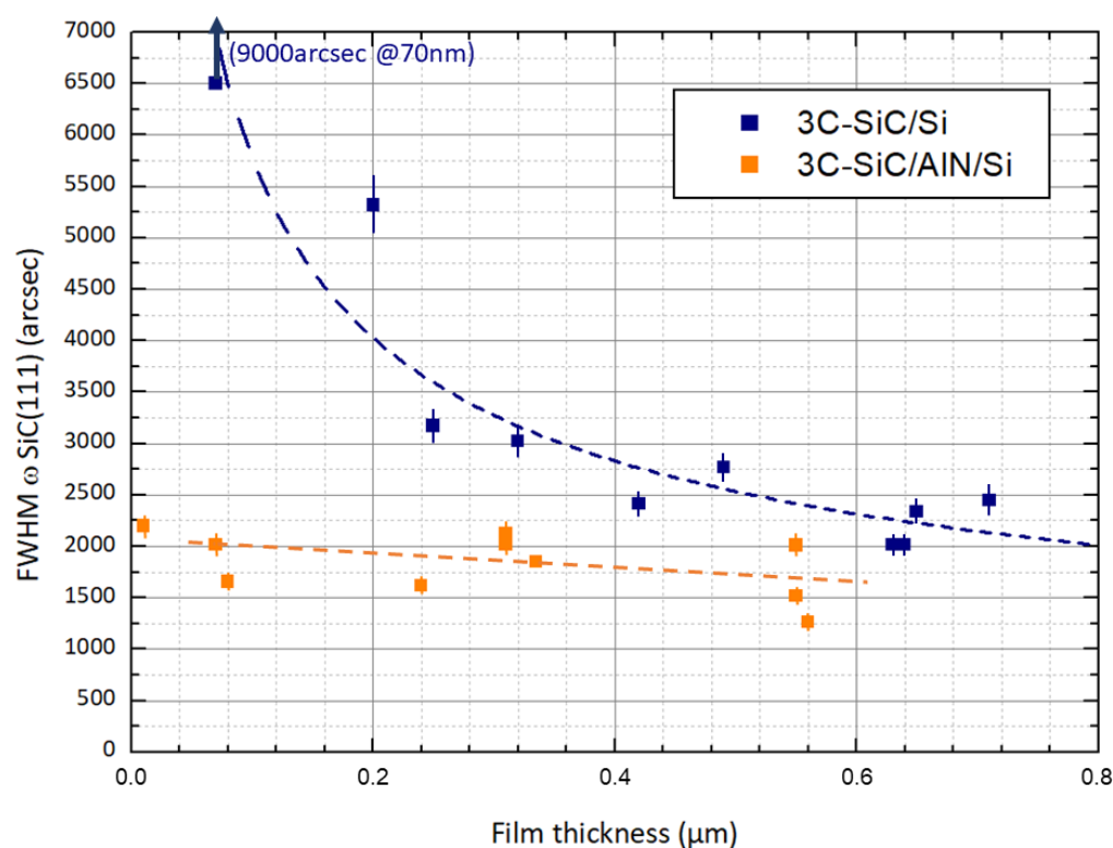
Figure 3. FWHMs recorded on the symmetric SiC(111) diffraction lines for 3C-SiC/AlN/Si (orange) and 3C-SiC/Si (blue) heterostructures. Dotted lines are guides for the eye.
