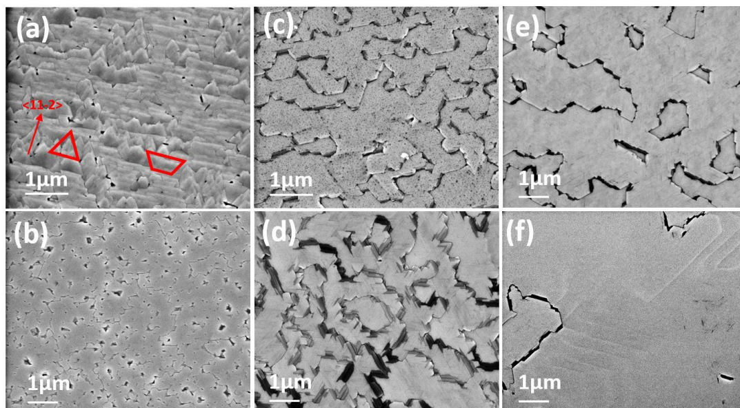
Figure 1. SEM micrographs: (a) 3C-SiC/AlN/Si(111) off axis —3 min of growth; (b) 3C-SiC/AlN/Si(111) on axis —3 min of growth; (c) 3C-SiC/AlN/Si(111) 4^\circ off axis —20 min of growth (SiC thickness—300 nm); (d) 3C-SiC/AlN/Si(111) on axis —20 min of growth (SiC thickness—320 nm); (e) 3C-SiC/AlN/Si(110) on axis —20 min of growth (SiC thickness—320 nm); (f) 3C-SiC/6H-SiC on axis —20 min of growth.
