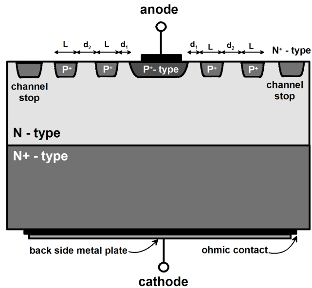
Figure 5: Schematic view of the PiN diode with a guard rings termination
