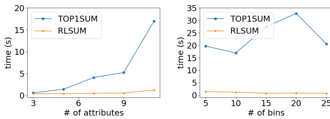
Figure 5: Average execution times (SDSS).
