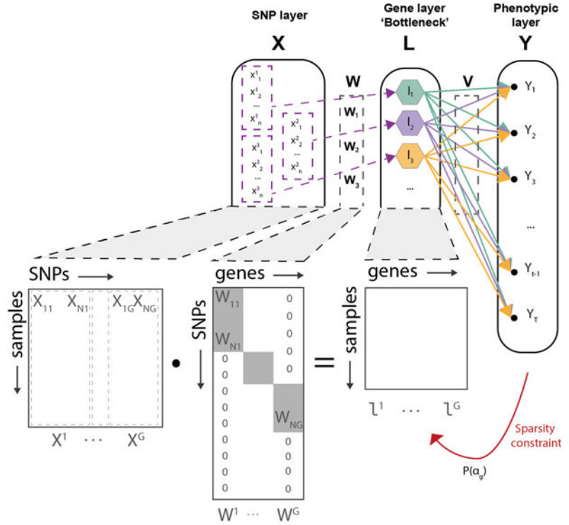
Fig. 6 Illustration of G2PSR SNP-gene grouping constraint and overall neural network architecture
