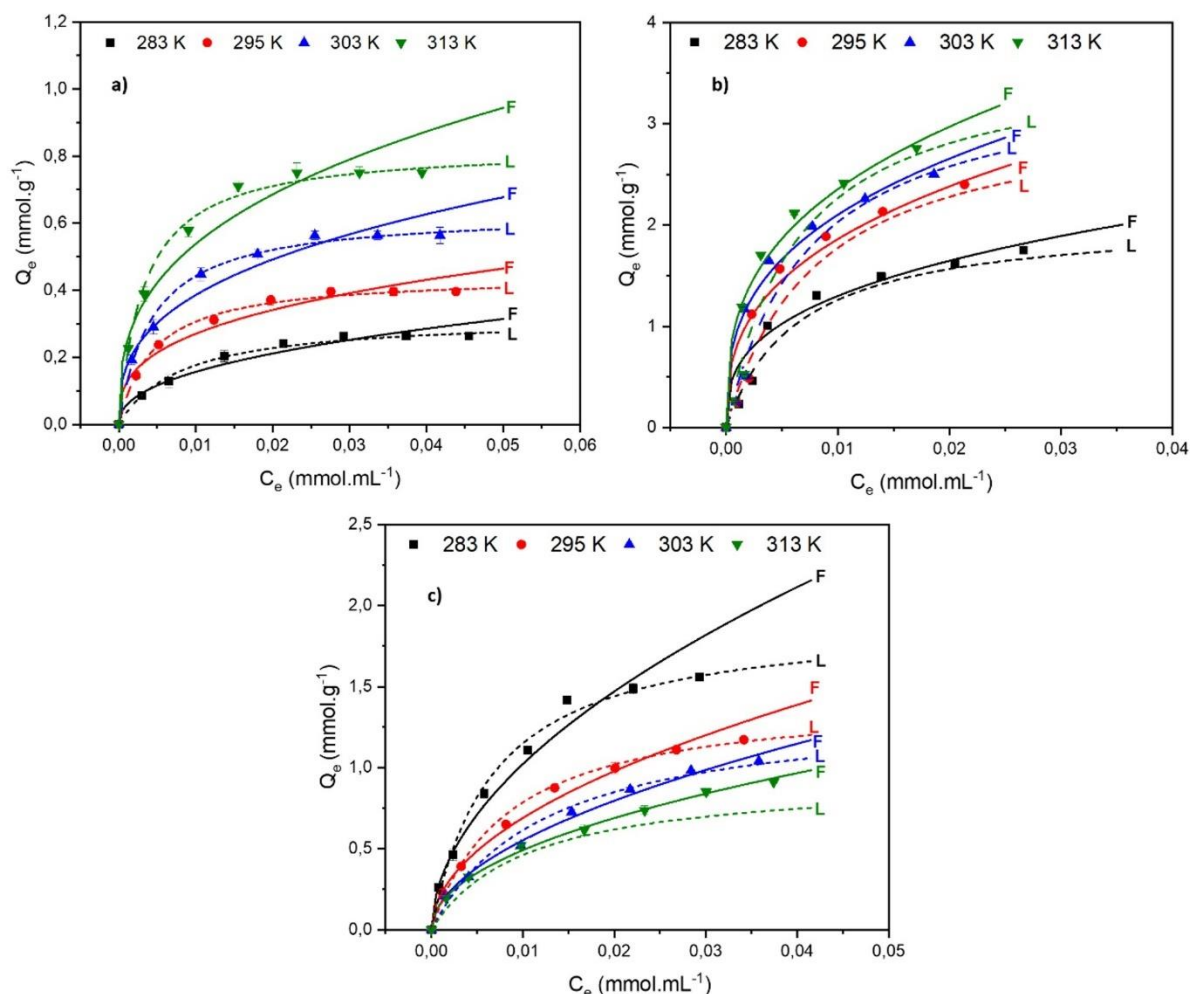
Fig.8. Comparison of the predicted adsorption isotherms and the experimental adsorption data for GSH onto (a) SBA-15-OH, (b) SBA-15-NH 2 , (c) SBA-15-SH adsorbents at 283, 295, 303 and 313 K, according to the Freundlich (F) and Langmuir (L) models.
