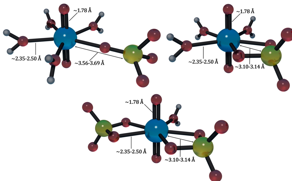
Fig. 3. To-scale idealised depictions of uranyl sulfate complexes. Structures are based on the DFT calculations of Hennig et al. [69]. Note how the monosulfate complex may contain either a monodentate or bidentate sulfate ion and how the U-S distance significantly differs between the two arrangements. Uranium is blue, oxygen red, sulfur yellow and hydrogen grey.
