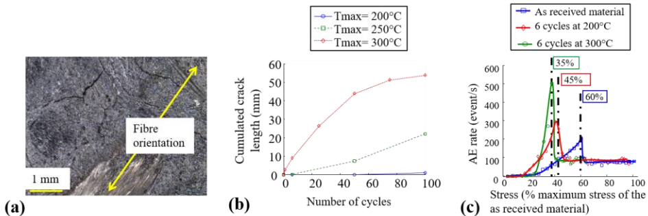
Figure 5: (a) A 2mm crack after 100 cycles at 250°C; (b) cumulated crack length; (c) Acoustic emission rate versus stress for the as received and thermally cycled material.
