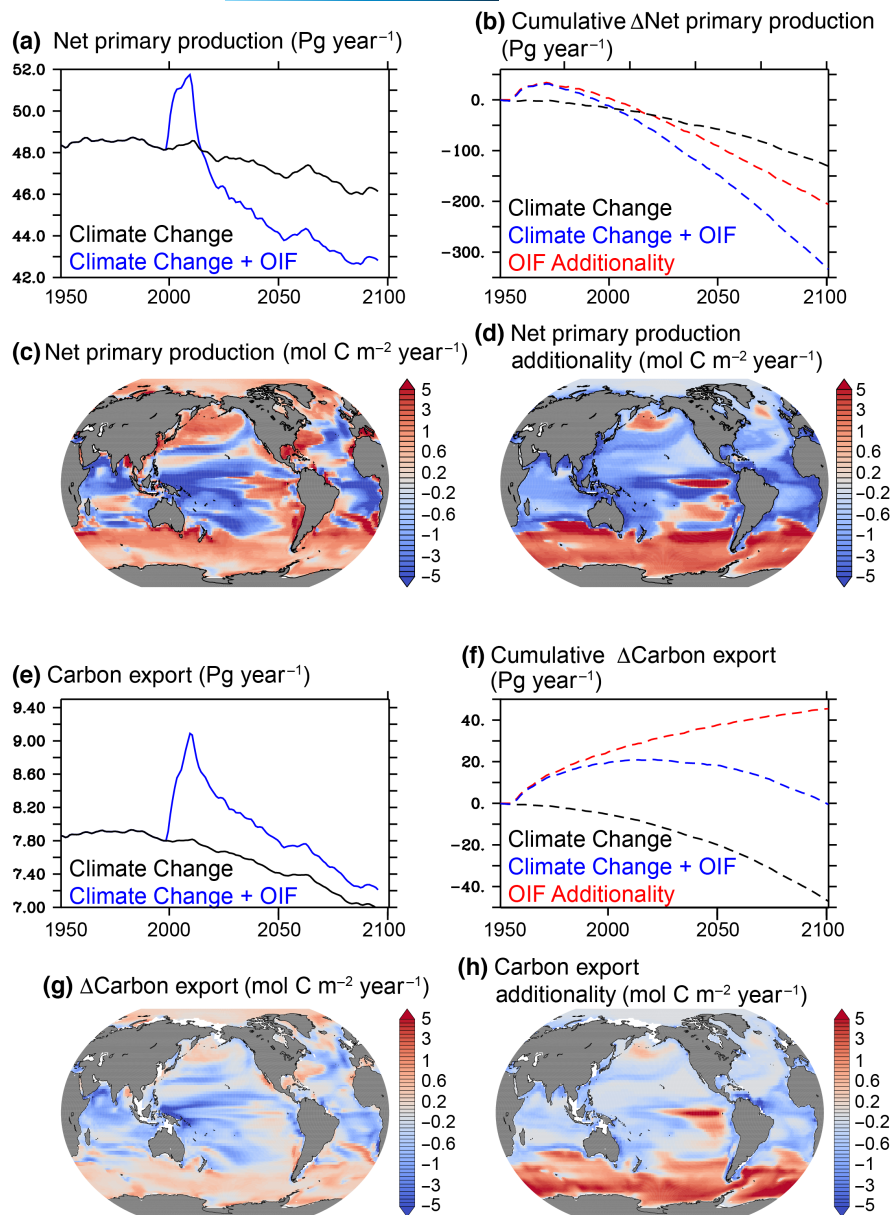
FIGURE 2 Time series of the evolution of (a) NPP (in \text{PgC year}^{-1} ) due to climate change (black) and climate change + OIF (blue) and (b) cumulative change in NPP (in \text{PgC} ) up to 2100 due to climate change (black dash) or climate change + OIF (blue dash), with OIF additionality is shown with red dash. Maps of (c) change ( \Delta ) in 2091–2100, relative to 1986–2005 in NPP due to climate change and (d) OIF additionality in NPP (both in \text{mol C m}^{-2} \text{ year}^{-1} ). Time series of the evolution of (e) carbon export (in \text{PgC year}^{-1} ) due to climate change (black) and climate change + OIF (blue) and (f) cumulative change in carbon export (in \text{PgC} ) up to 2100 due to climate change (black dash) or climate change + OIF (blue dash), with OIF additionality is shown with red dash. Maps of (g) change ( \Delta ) in 2091–2100, relative to 1986–2005 in carbon export due to climate change and (h) OIF additionality in carbon export (both in \text{mol C m}^{-2} \text{ year}^{-1} ). NPP, net primary production; OIF, ocean iron fertilization.
