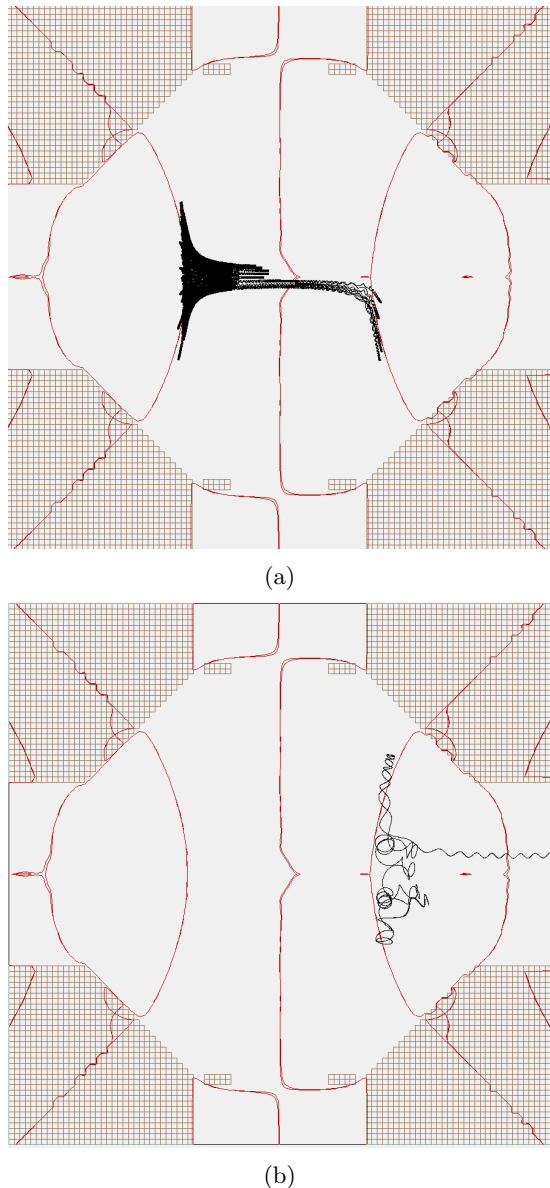
FIG. 8: trajectories computed with SIMION. (a) q = 8 ; (b) q = 1 . \text{Ar}^{8+} ions are trapped inside the magnetic field distribution.
