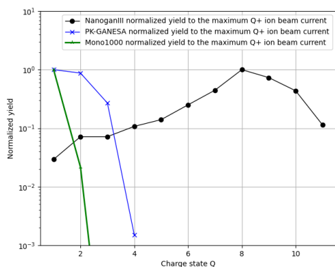
FIG. 1: Charge state distribution of Ar ions normalized to the maximum current peak for NANOGANIII (Black, a maximum peak current of 150 \mu\text{A} [10]); PK-GANESA (blue, maximum peak current of 190 \mu\text{A} [5]); and MONO1000 (green, maximum peak current of 501 \mu\text{A} ).
