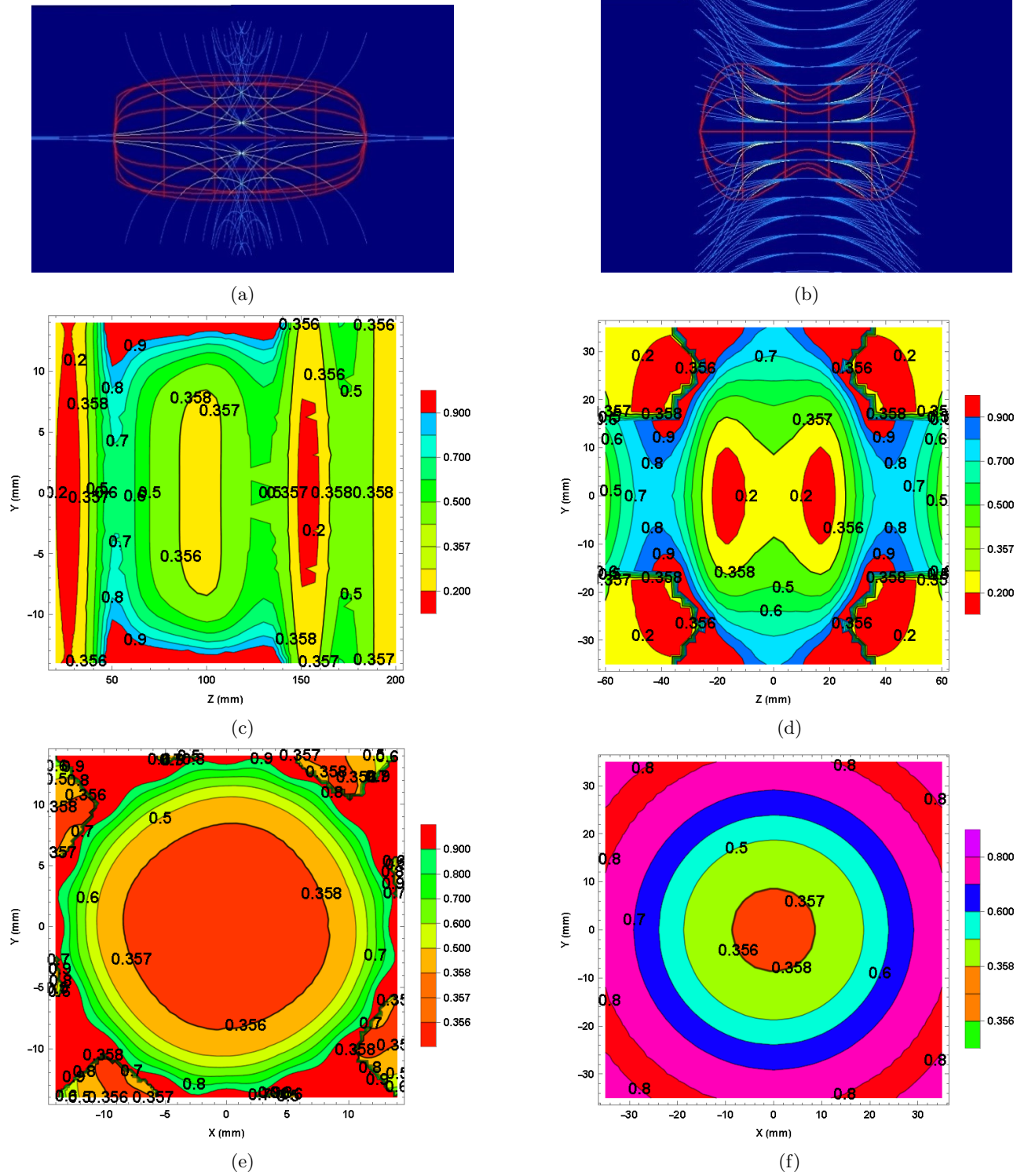
FIG. 2: Magnetic topology with resonance zone for (a) NANOGANIII and (b) PK-GANESA; Red lines belong to the ECR resonance surface, where the magnetic-field related electron-cyclotron resonance matches the microwave, namely 10 GHz; Blue lines correspond to magnetic-field lines and the yellow ones are those crossing the ECR resonance volume. Magnetic-field contour plots: in the vertical plane which contains the source axis for (c) NANOGANIII and (d) PK-GANESA; in the transverse plane at the centre of the source on the longitudinal axis for (e) NANOGANIII and (f) for PK-GANESA. The numbers correspond to the field values in T.
