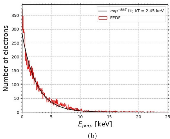
FIG. 3: EEDF of trapped electrons after 20 \mu\text{s} of simulation for 10 GHz 800 W RF heating (a) NANOGANIII and (b) PK-GANESA. The scale difference on the y-axis is related to the numbers of the trapped electrons of both simulations (3 % for (a) as compared with 30 % for (b) of the same statistics of initial electrons).
