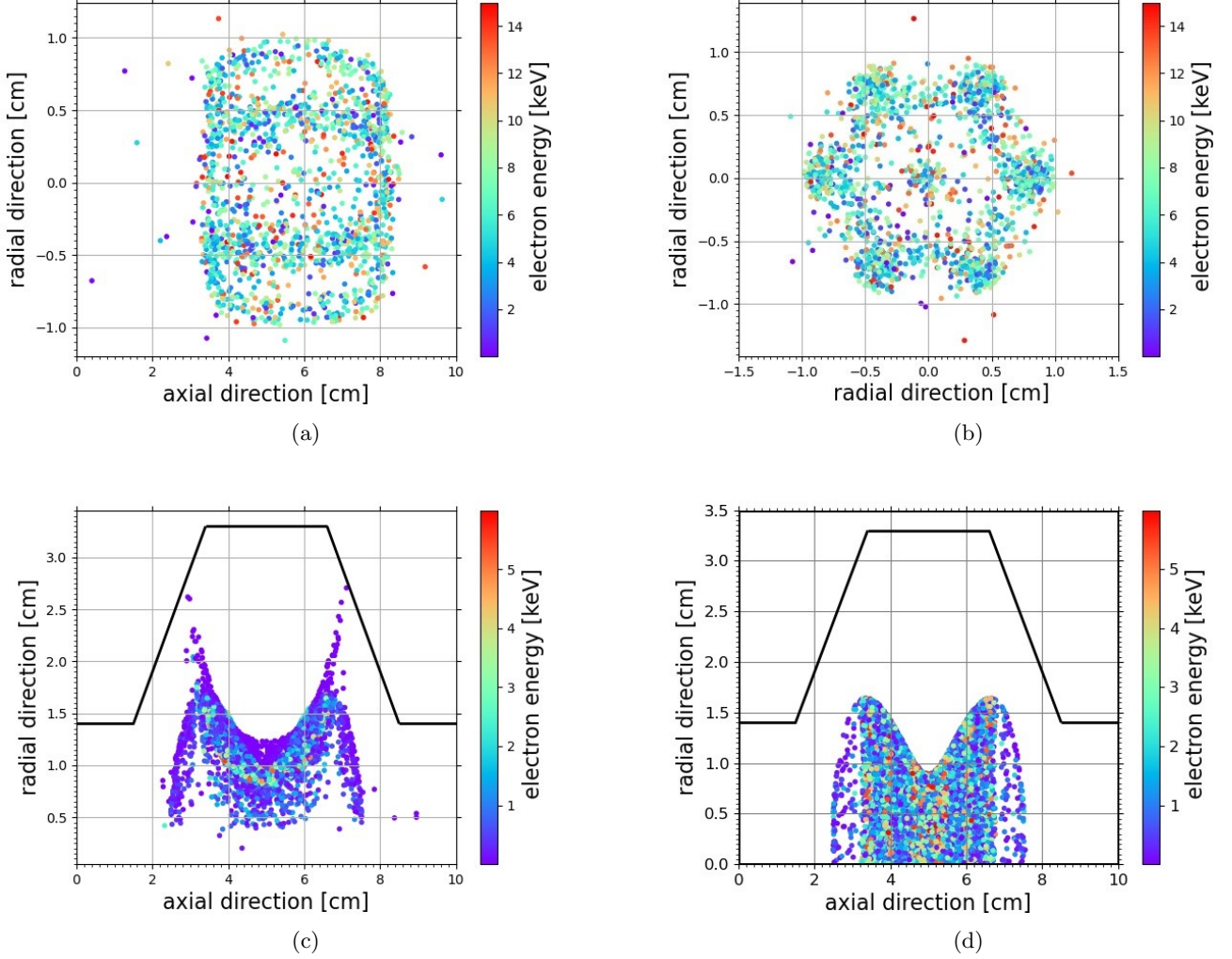
FIG. 5: Electron spatial distribution of non-lost electrons at 20 \mu\text{s} : (I) NANOGANIII final distribution (a) axial view (b) radial view and (II) PK-GANESA (c) final distribution axial view and (d) initial distribution axial view; Note that both distributions for PK-GANESA are radially symmetric. Hence they are not presented in the radial plane, orthogonal to the axial direction.
