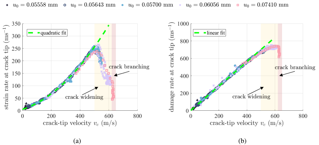
Figure 6: The evolution of the strain and the damage rates around the crack tip as a function of the crack-tip velocity. A quadratic relationship is found between the strain rates and the tip velocities (a). A linear relationship is found between the damage rates and the tip velocities (b).
