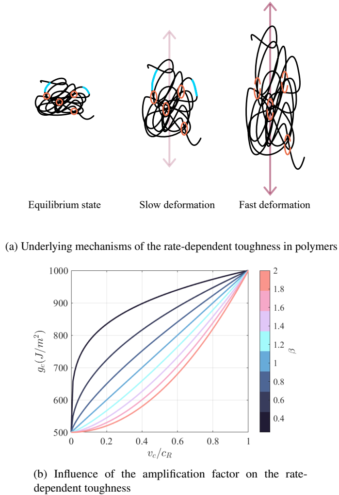
Figure 3: Rate-dependent toughness: the underlying mechanisms (a) in polymers and the influence of the amplification factor (b) – Equation (19).
