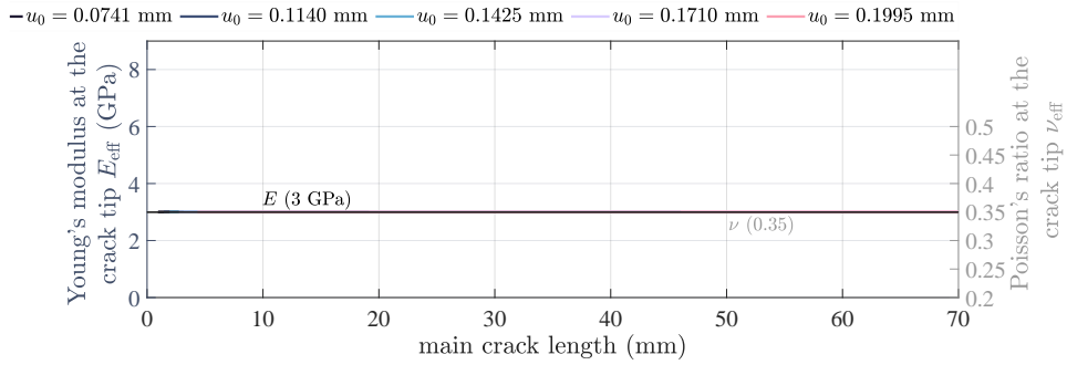
Figure 17: No stiffening at the crack-tip in the material with damage-rate dependent toughness.
