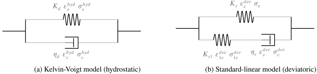
Figure 2: Illustration of the viscoelastic model of the bulk: (a) Kelvin-Voigt model for the hydrostatic part and (b) Standard linear model for the deviatoric part.
