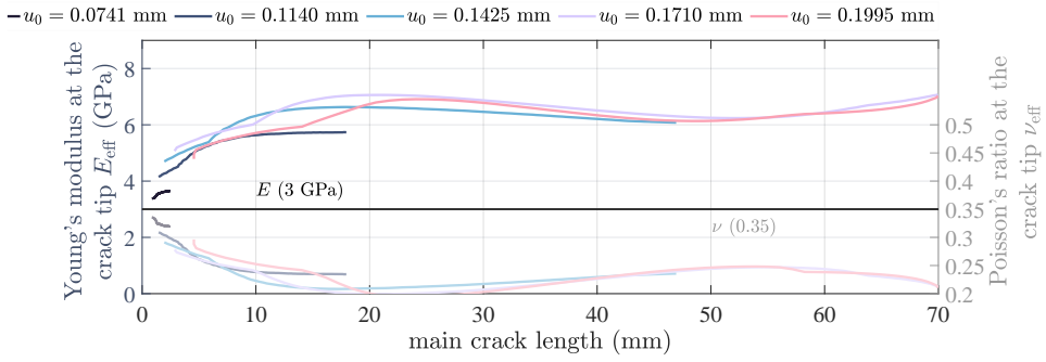
Figure 14: Effective stiffening at the crack-tip in the viscoelastic material with \zeta = 0 .
