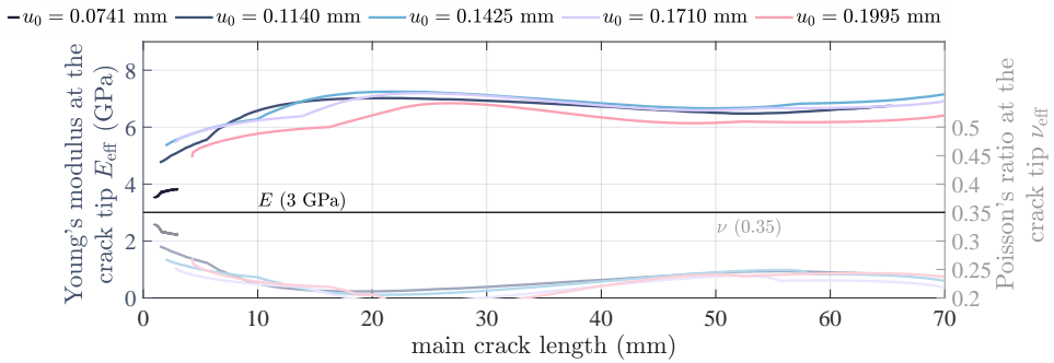
Figure 15: Effective stiffening at the crack-tip in the viscoelastic material with \zeta = 1 .
