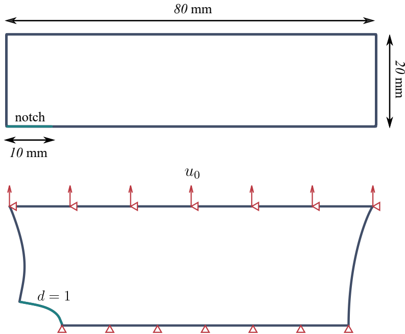
Figure 4: Half-strip geometry (top) and applied boundary conditions (bottom) for the uniform displacement strip.
