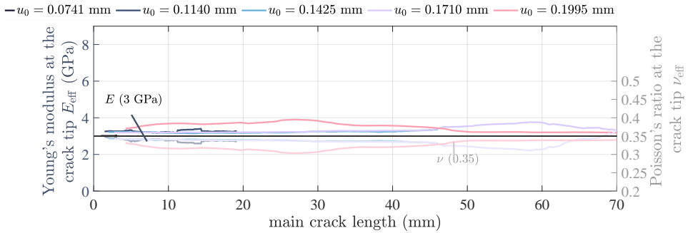
Figure 16: Effective stiffening at the crack-tip in the material with strain-rate dependent toughness.
