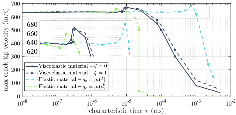
Figure 11: Influence of the models' characteristic time ( \tau_v ) on the maximum crack-tip speed (imposed vertical displacement u_0 = 0.0741 mm).
