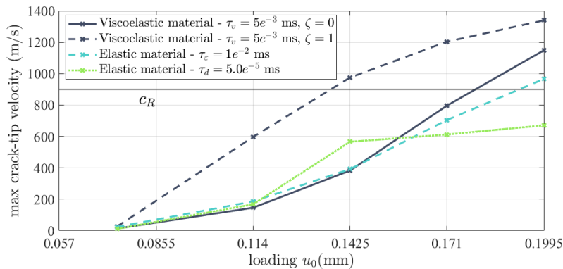
Figure 12: Maximum crack-tip velocities at multiple loadings.
