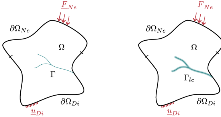
Figure 1: Regularised representation of a crack in a two-dimensional case, sharp crack (left) and regularised representation through phase-field (right). Ne and Di subscripts stand for Neumann and Dirichlet boundary conditions respectively.
