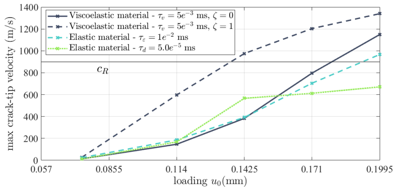
Figure 12: Maximum crack-tip velocities at multiple loadings.
