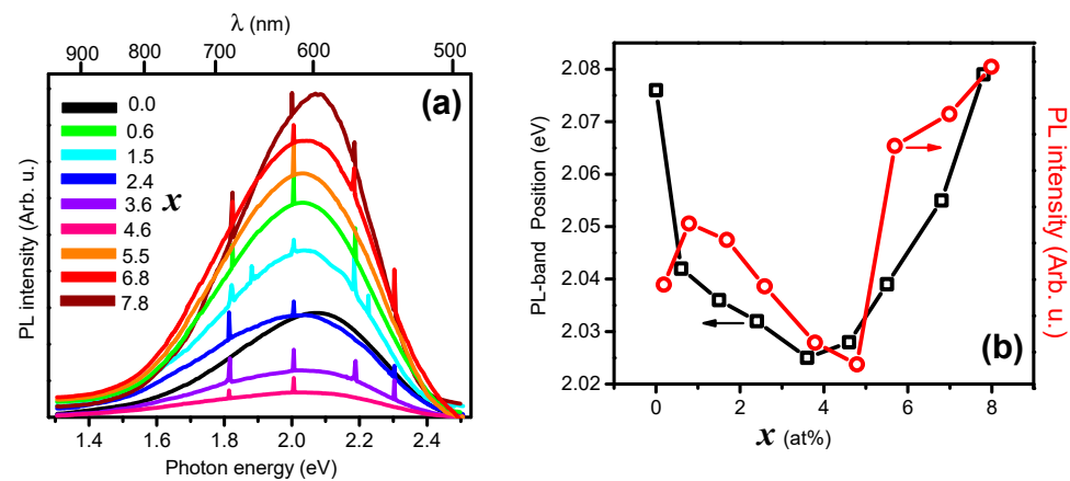
Figure 6. (a) Photoluminescence spectra of all the set of Cd_{1-x}Er_xSe samples. (b) Energy position of the PL band maximum (left axis) and PL band intensity (right axis) versus x .
