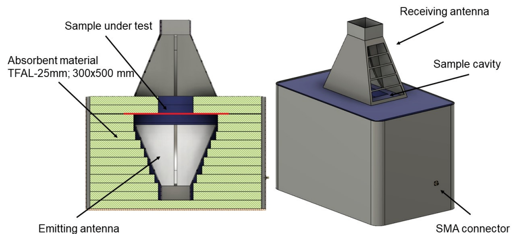
Figure 7. Cross-sectional view of the prototype system.
