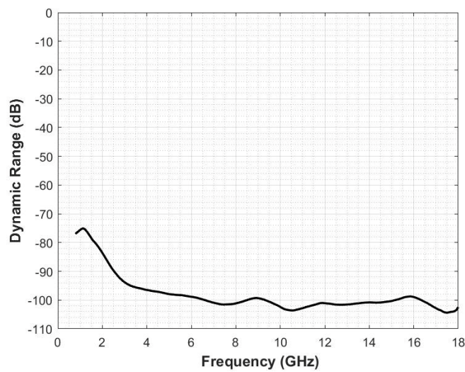
Figure 9. Measured dynamic range of the system with a 2 mm thick aluminum sample.
