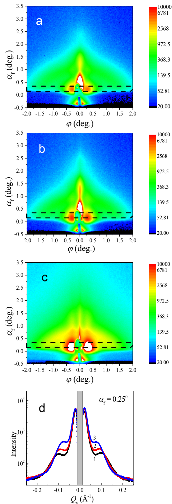
Figure 3. (a) The two-dimensional GISAXS intensity maps from the samples SiO 2 (38 at.% Co)/Si (a), SiO 2 (54 at.% Co)/Si (b), and SiO 2 (82 at.% Co)/Si (c). The dashed horizontal lines indicate the integration regions for the one-dimensional profiles shown on (d) panel. (d) The scattering intensity profiles along \phi direction at \alpha_f = 0.25^\circ for SiO 2 (38 at.% Co)/Si—curve 1, SiO 2 (54 at.% Co)/Si—curve 2, and SiO 2 (82 at.% Co)/Si—curve 3. The gray area corresponds to the beamstop shadow.
