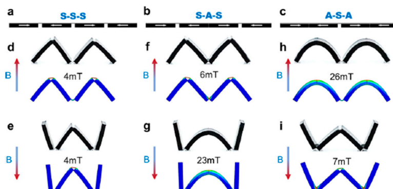
Figure 11. A combination of symmetric (S) and asymmetric (A) joints [49]. (a) S–S–S (b) S–A–S (c) A–S–A. (d–i) Simulated deformations for the joint types in (a–c) with positive (d,f,h) and negative (e,g,i) magnetic field.
