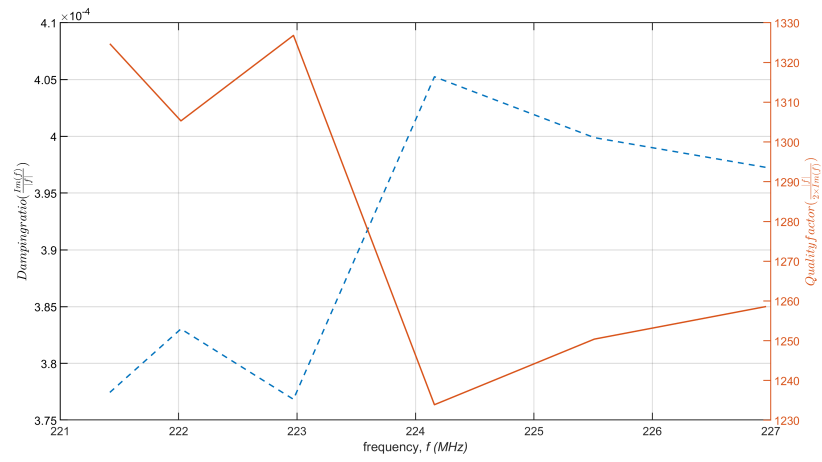
Figure 16. Damping ratio (blue dashed-line) and quality factor (red line) as a function of frequency.
