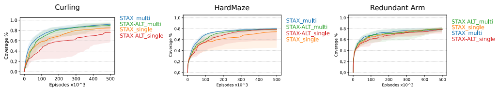
Figure 7: Median coverage with respect to the given evaluation budget reached by STAX against the ablated versions of the algorithm. The shaded areas represent the 10 and 90 percentile calculated over 15 seeds.
