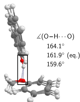
Fig. 7 Equilibrium geometry of c2NA_O at the B3LYP-D3 abc (BJ)/def2-QZVP level superimposed with normal mode displacements in opposing directions along \nu_{101} which modulates the O–H \cdots O angle.
