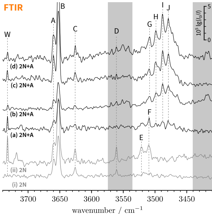
Fig. 3 FTIR decadic absorbance spectra ( \lg(I_0/I) ) of bare 2-naphthol expansions (i-ii, grey) and 2-naphthol and anisole co-expansions (a-d, black) with varying concentrations and water content. An extended version covering a broader spectral range can be found in the ESI† (Fig. S1). The overall signal enhancement from traces (a) and (b) to (c) and (d) illustrates the extended absorption path length in the new setup. 31 Note that bands F and G partially overlap (see Section 4.1.2).
