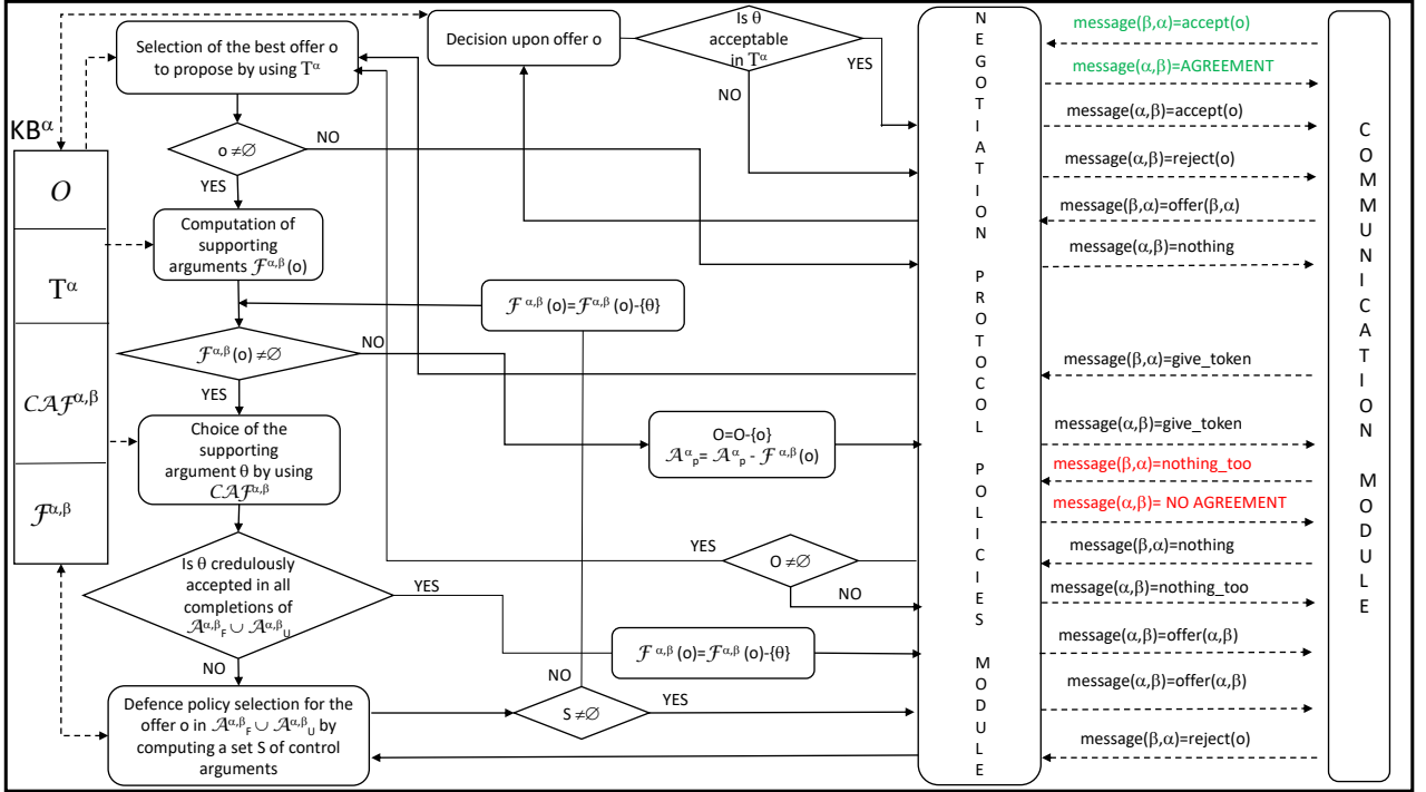
Figure 6: Architecture of a negotiating agent \alpha
