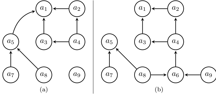
Figure 3: Some completions of the previous CAF
