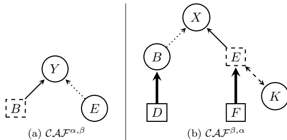
Figure 5: The opponent modelling of agents \alpha and \beta
