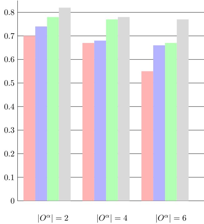
Figure 10: Agreement rate (rounded to 10^{-2} ) for |O^\alpha| \in \{2, 4, 6\} , and \text{densContrAtt} is 0.03 (red), 0.05 (blue), 0.10 (green) or 0.20 (gray), for theories with \text{density} = 0.15
