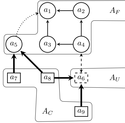
Figure 2: Example of a CAF
