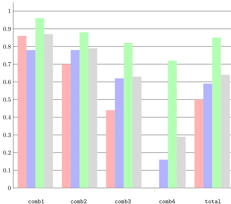
Figure 12: Agreement rate (rounded to 10^{-2} ) for the different combinations of parameters, for density = 0.15, 6 offers, and densContrAtt = 0.05, the size of the shared part of theories is 0.25 (red), 0.50 (blue), or 0.75 (green), and the aggregation of the three different sizes (gray)
