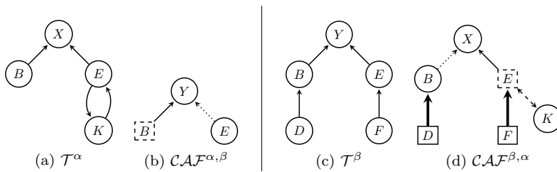
Figure 7: The theories of agents \alpha and \beta before the negotiation
