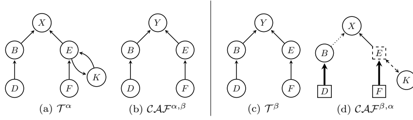
Figure 8: The theories of agents \alpha and \beta after the negotiation
