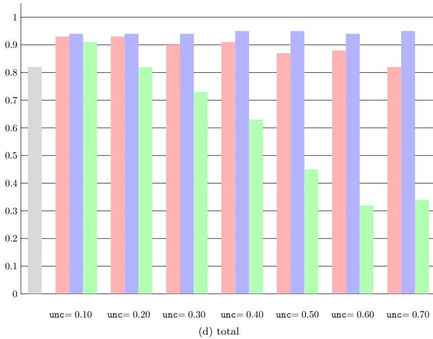
Figure 13: Agreement rate (rounded to 10^{-2} ) of negotiations for theories with density = 0.15 , densContrAtt = 0.05 , and 4 offers, unc \in \{0.10, 0.20, 0.30, 0.40, 0.50, 0.60, 0.70\} with parameters Arg in red, Att in blue and Both in green, and the aggregate in gray
