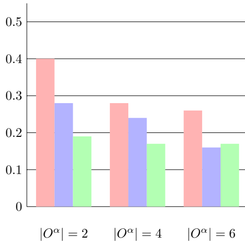
Figure 9: Agreement rate (rounded to 10^{-2} ) for negotiations with theories without control arguments, for |O^\alpha| \in \{2, 4, 6\} , and density is 0.10 (red), 0.15 (blue) or 0.20 (green)
