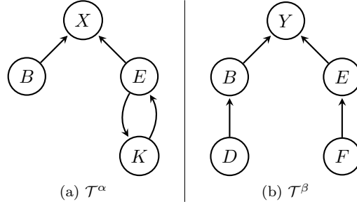
Figure 4: The personal theories of agents \alpha and \beta
