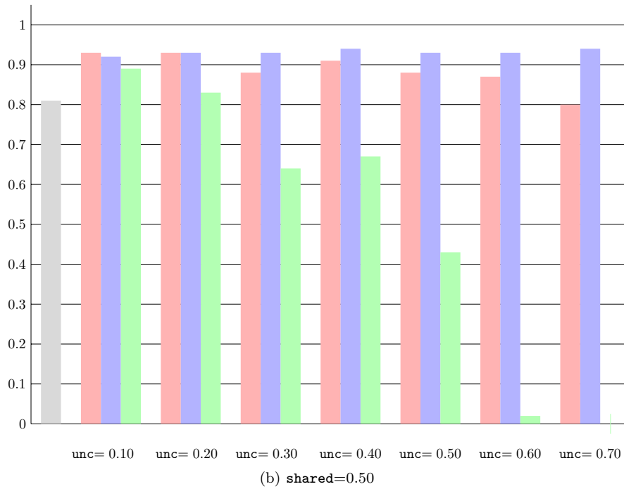
Figure 13: Agreement rate (rounded to 10^{-2} ) of negotiations for theories with density = 0.15, densContrAtt = 0.05, and 4 offers, unc \in {0.10, 0.20, 0.30, 0.40, 0.50, 0.60, 0.70} with parameters Arg in red, Att in blue and Both in green, and the aggregate in gray
