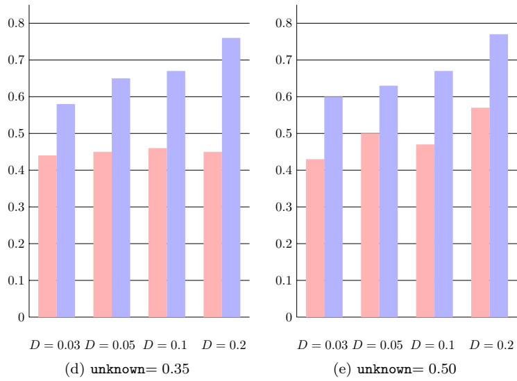
Figure 14: Agreement rate (rounded to 10^{-2} ) for negotiations with theories with density 0.15, parameter unknown is 0 (Fig. 14a), 0.15 (Fig. 14b), 0.25 (Fig. 14c), 0.35 (Fig. 14d) or 0.50 (Fig. 14e), numContrArg is 3 (red) or 6 (blue), and densContrAtt is D \in \{0.03, 0.05, 0.1, 0.2\}
