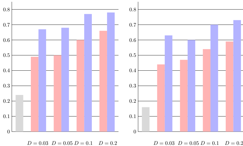
Figure 11: Agreement rate (rounded to 10^{-2} ) for negotiations with theories with density 0.15 (left) or 0.20 (right), numContrArg is 0 (gray), 3 (red) or 6 (blue), and densContrAtt is D \in \{0.03, 0.05, 0.1, 0.2\}
