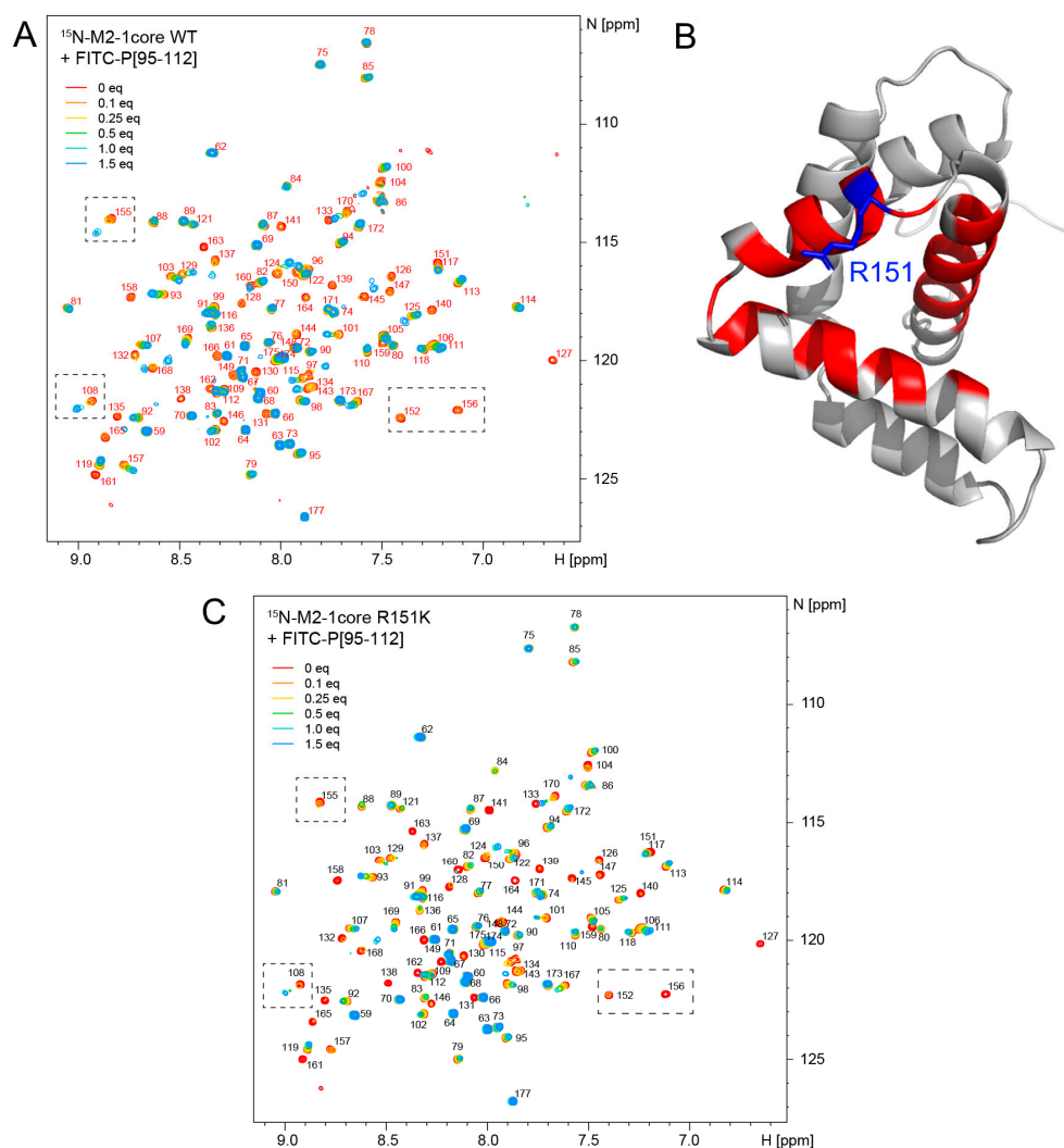
Figure 4. The M2-1-P complex displays motions at the \mu s–ms time scale. (A) Binding of the FITC-P 95–112 peptide to ^{15}\text{N} -labeled M2-1core domain was followed by 2D NMR ( ^1\text{H} frequency 700 MHz, temperature 298 K). Amide signals are annotated with the corresponding residue number. Increasing amounts (0.1 to 1.5 molar equivalents) of FITC-P 95–112 peptide were added to 100 \mu\text{M} WT M2-1core and a ^1\text{H} - ^{15}\text{N} BTROSY spectrum was acquired at each titrating point. Saturation was reached at a peptide-protein molar ratio of 1.5:1. (B) The signals of nearly all residues belonging to the P-binding site remain broad at the last titration point. They are mapped in red on the structure of M2-1core (PDB 2L9J). (C) Titration of ^{15}\text{N} -labeled M2-1core R151K mutant by 0.1 to 1.5 molar equivalents FITC-P 95–112 peptide is followed by measuring the ^1\text{H} - ^{15}\text{N} BTROSY spectra.
