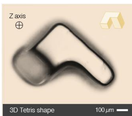
Figure 4: example of an unsupported true 3D Tetris shape fabricated using a sequentially interrupted flow (irradiation: green laser power of 1 W and exposure time of 0.4 second).
