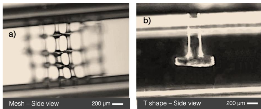
Figure 3: supported true single shot 3D shapes: a) mesh inclined at 45° to the channel axis and b) T shape, both anchored inside a microfluidic channel of a 1 mm x 1 mm cross section (irradiation: green laser power of 1W and exposure time of 0.4 second).
