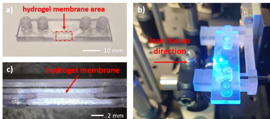
Figure 6: a) 3D printed microfluidic chip with 2 channels, b) microfluidic chip under laser illumination to photopolymerize an hydrogel membrane, c) side-view of the microfluidic chip with the hydrogel membrane separating the 2 channels.
