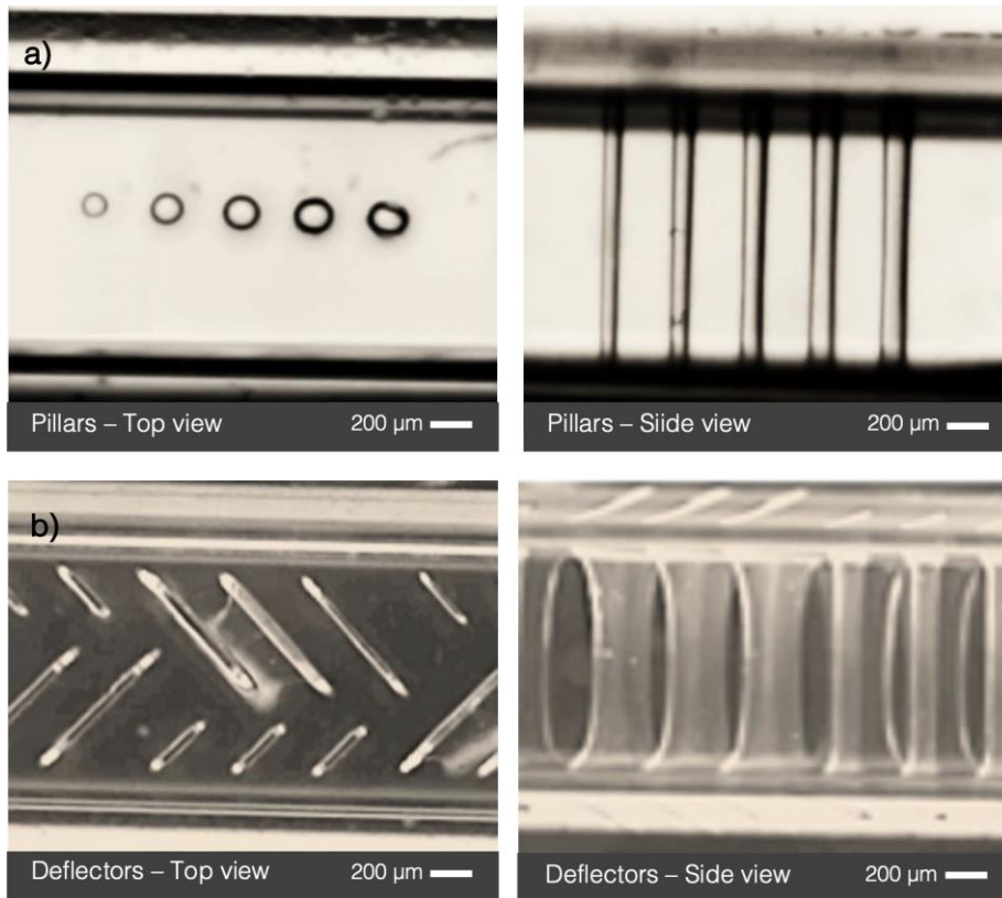
Figure 2: a) pillars of varying diameters and b) deflectors to be used as fluid mixers, both anchored inside a microfluidic channel of a 1 mm x 1 mm cross section (irradiation: green laser power of 1W and exposure time of 0.4 second).
