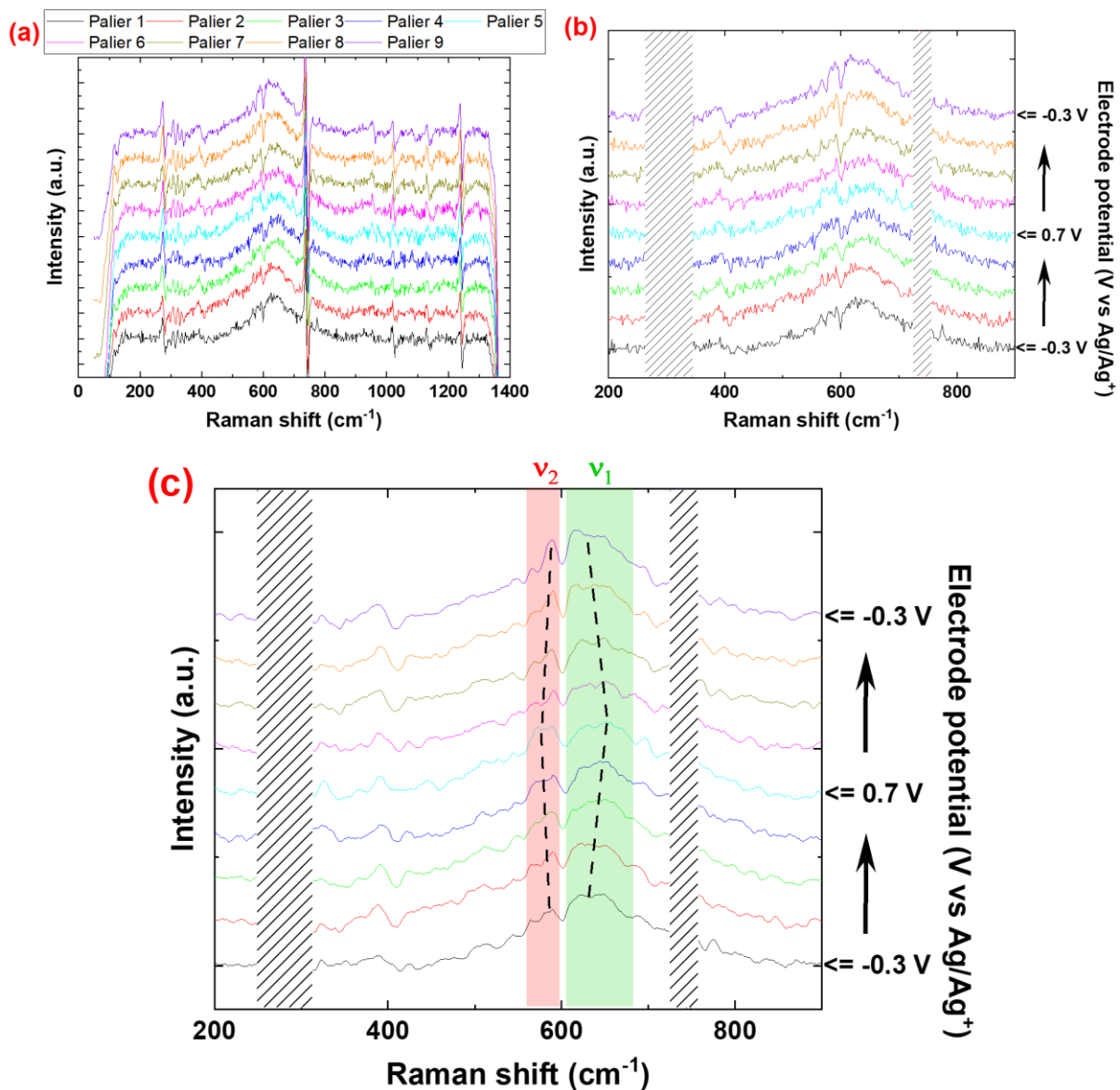
Figure 9 : Raman spectra of the MnO 2 electrode in pure EMImTFSI, (a) between 50 and 1400 cm -1 after removal of EMImTFSI bands, (b) between 200 and 900 cm -1 and (c) after smoothing noise. Hatched parts cover defects after the removal of EMImTFSI spectrum, for a better legibility.
