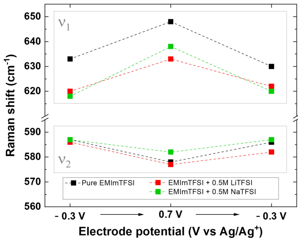
Figure 11 : Evolution of the positions of \nu_1 and \nu_2 bands versus the charge state of the electrode and the electrolyte used.
