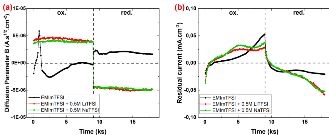
Figure 4 : Evolution of (a) the diffusion parameter and (b) the residual current. Oxidation and reduction are separated by the vertical dotted line.
