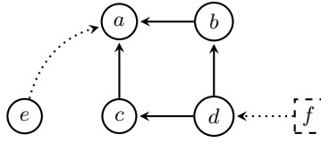
Fig. 6: The IAF \mathcal{I}
