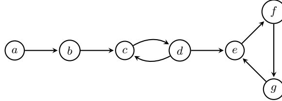
Fig. 1: An Example of AF \mathcal{F}
