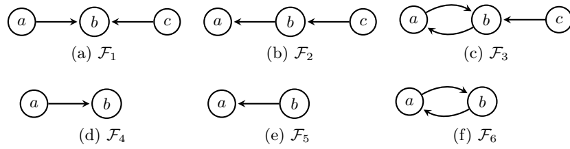
Fig. 5: The Completions of r\mathcal{I}
