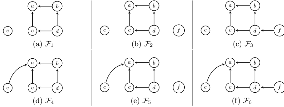
Fig. 7: The Completions of \mathcal{I}
