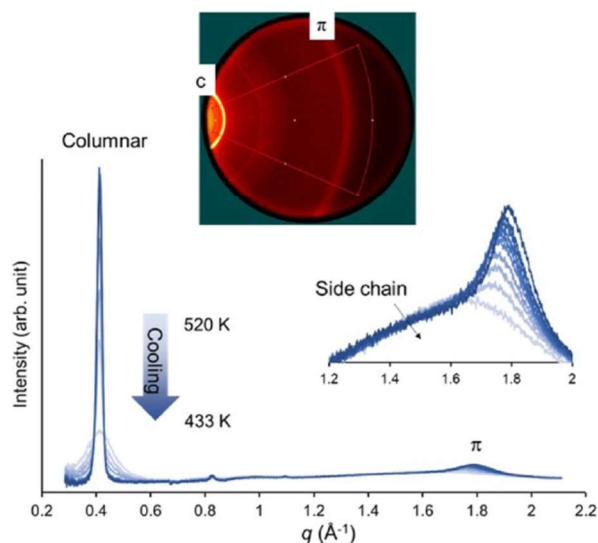
FIG. 1. X-ray scattering curves of PNP measured during cooling from the isotropic liquid state. The 0.41 Å -1 peak results from intercolumnar scattering, the 1.8 Å -1 peak results from \pi - \pi scattering, and the broad feature near 1.5 Å -1 results from the correlation between the side chains of the aromatic core. Insets: a typical 2D scattering pattern and an enlarged view of the \pi scattering peak.
