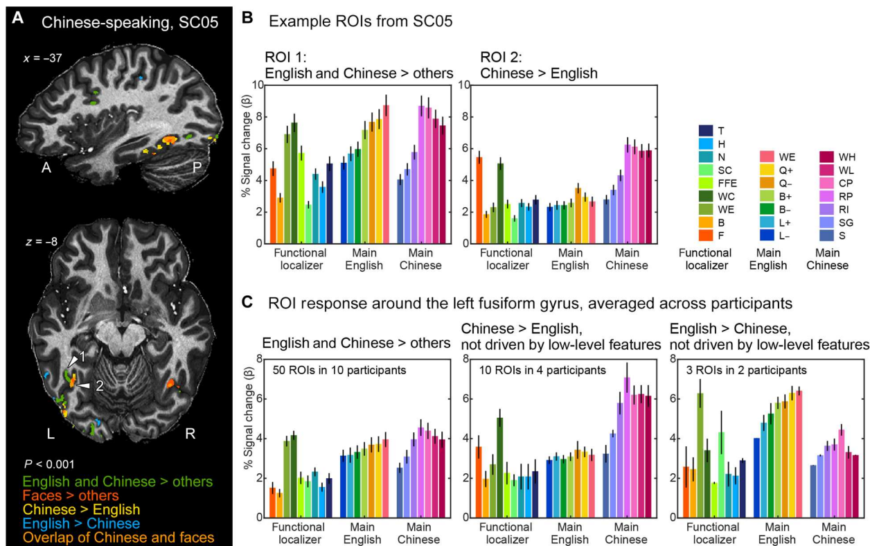
Fig. 7. Word-specific and language-specific activation in English-Chinese bilingual readers. (A) Example of ventral occipitotemporal activation in a representative participant (SC05; P < 0.001 uncorrected; see fig. S6 for the maps of all 10 participants). The word-specific and face-specific clusters were defined with the localizer (English and Chinese words > faces, bodies, houses, and tools; faces > bodies, houses, tools, and English and Chinese words). The Chinese- and English-specific clusters were defined with the main fMRI runs (Chinese words > English words and vice versa). Note the overlapping sensitivity for Chinese words and for faces (orange color) in ROI 2 (white arrowheads) and a symmetrical right-hemispheric ROI. (B) Activity profile of two example ROIs from participant SC05, labeled with white arrowheads in (A). ROI 1 shows shared responses to English and French words and corresponding word-similarity effects, while ROI 2 is sensitive to Chinese stimuli and faces. (C) Group-averaged activity profiles of bilingual word-specific ROIs around the left fusiform gyrus (left), with preference for Chinese stimuli (middle), or with preference for English stimuli (right). Note the strong response to faces (red bar) in the Chinese-specific ROIs (middle). See figs. S7 and S8 for all individual ROIs.
