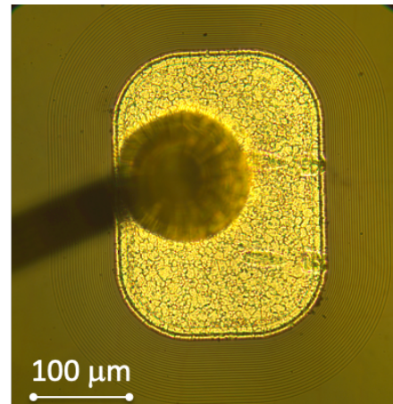
Fig. 13 Photograph of the diode with the 50 μm (diameter) gold ball bonding.
