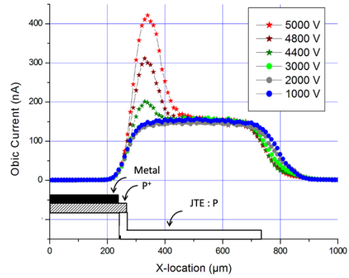
Fig. 8 1D-sweeping OBIC measurements were performed on a diode with a 500 \mu\text{m} MESA JTE protection at various voltages.
