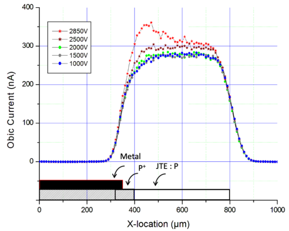
Fig. 5 OBIC current measured at different increasing voltages on device #2. A 10 \mu\text{m} step for the line was used.
