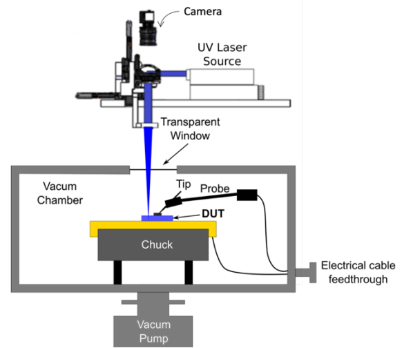
Fig. 2 Schematic of the experimental OBIC bench
