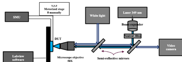
Fig. 11 Schematic representation of the enhanced micro-OBIC testbench.
