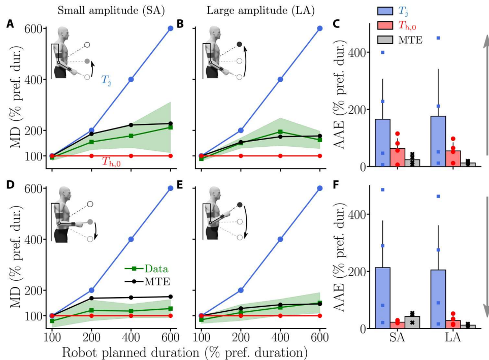
Fig. 6. Chosen relative MD of participants when assisted by the exoskeleton with different T_j values. Average data are represented by green lines with SD represented by green shaded areas. Outputs of different simulated motor strategies are depicted as follows: blue, simulation results with MD = T_j ; red, simulation results with MD = T_{h,0} ; black, simulation results under the MTE hypothesis. (A and B) Relative MD of upward movements for the SA (A) and the LA (B). (C) AAEs of the different hypothetical strategies for both SA and LA for upward movements. (D and E) Relative MD of downward movements for the SA (D) and the LA (E). (F) AAEs of the different modeled strategies for both SA and LA for downward movements.
