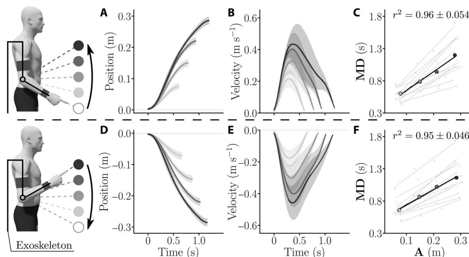
Fig. 3. General kinematics averaged across all participants in the transparent exoskeleton for both upward and downward movements. (A and D) Averaged positions for upward (A) and downward (D) movements across population. SDs are depicted as shaded areas. (B and E) Averaged velocities for upward (B) and downward (E) movements across population. (C and F) Amplitude–MD linear regressions for each participant (gray) for upward (C) and downward (F) movements. The average behavior of participants is shown in black. The mean correlation coefficient and its SD across participants are reported for each movement direction.
