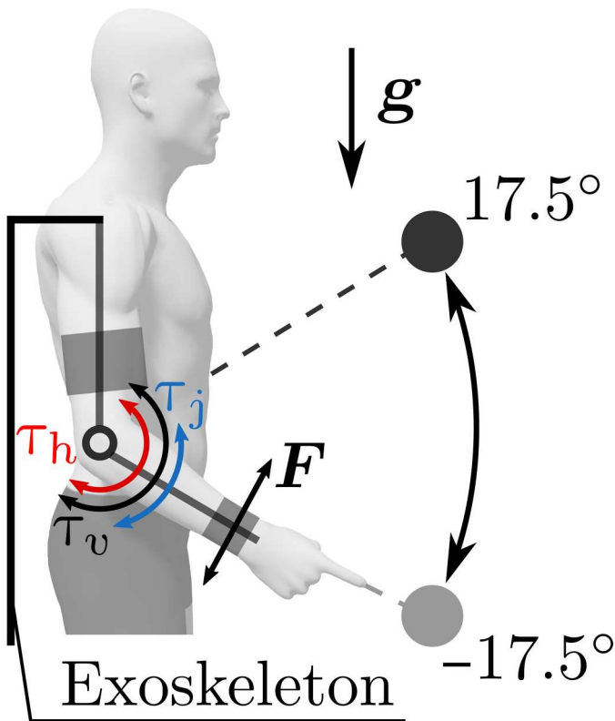
Fig. 1. Illustration of the task and the different input torques involved. The term \tau_j is the torque provided by the robot as a biological movement assistance (here a minimum jerk trajectory of duration T_j ), which is activated as long as the participant does not outpace the planned trajectory. The term \tau_h is the net torque produced by the human muscles ( \tau_h = 0 when the participant is inactive). The term \tau_v is a viscous-like torque applied by the robot, which replaces \tau_j as soon as the participant outpaces the planned trajectory. F is the measured interaction force.
