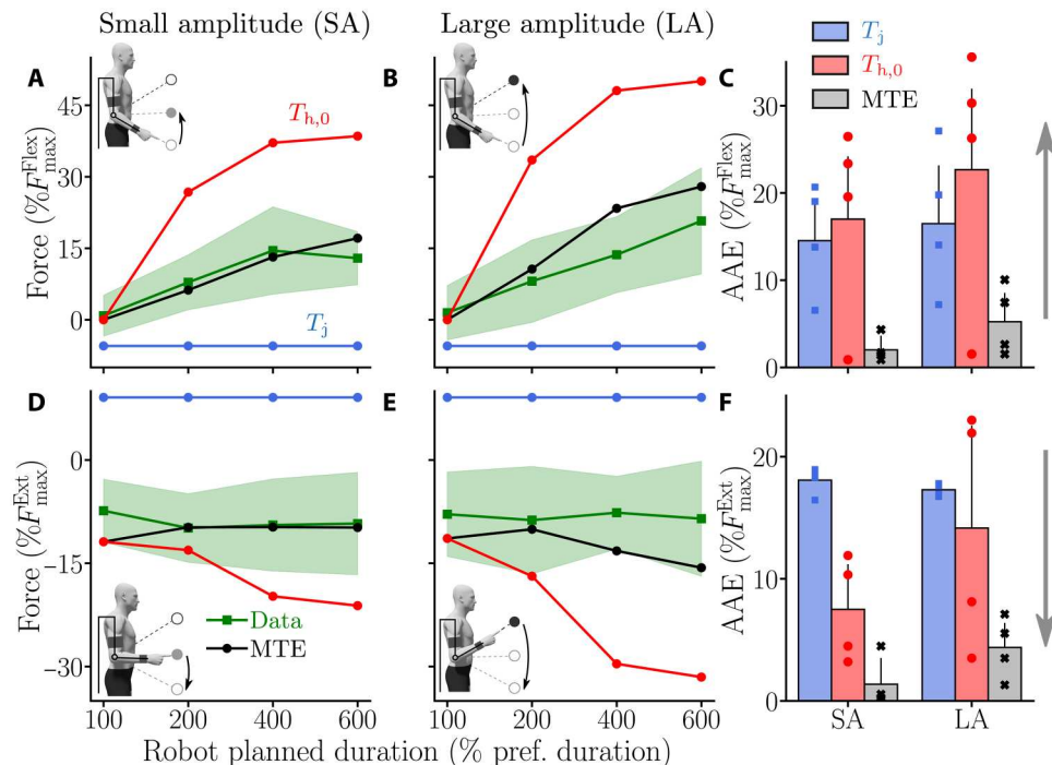
Fig. 7. Maximum interaction force when the participant is assisted by the exoskeleton with different T_j values. Average data are represented by green lines and SDs as green-shaded areas. Outputs of different simulated motor strategies (based on the dynamics from Eqs. 8 and 10; see Methods) are depicted as follows: blue, simulation results with MD = T_j ; red, simulation results with MD = T_{h,0} ; black, simulation results under the MTE hypothesis. (A and B) Maximum interaction force during upward movements for the SA (A) and the LA (B). (C) AAE of the different modeled strategies for both SA and LA for upward movements. (D and E) Maximum interaction force during downward movements for the SA (D) and the LA (E). (F) AAE of the different modeled strategies for both SA and LA for downward movements.
