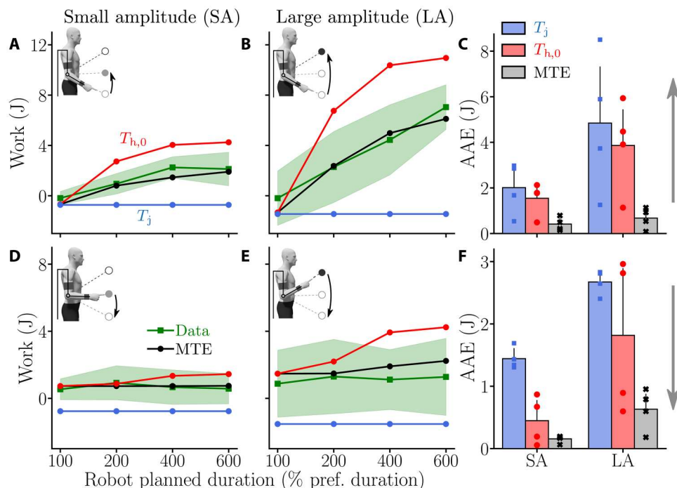
Fig. 8. Work of the interaction force when the participant is assisted by the exoskeleton with different T_j values. Average data are represented by green lines, and SDs are represented as green shaded areas. Outputs of different simulated motor strategies are depicted as follows: blue, simulation results with MD = T_j ; red, simulation results with MD = T_{h,0} ; black, simulation results under the MTE hypothesis. (A and B) Work for upward movements for the SA (A) and the LA (B). (C) AAE of the different modeled strategies for both SA and LA for upward movements. (D and E) Work for downward movements for the SA (D) and the LA (E). (F) AAE of the different modeled strategies for both SA and LA for downward movements.
