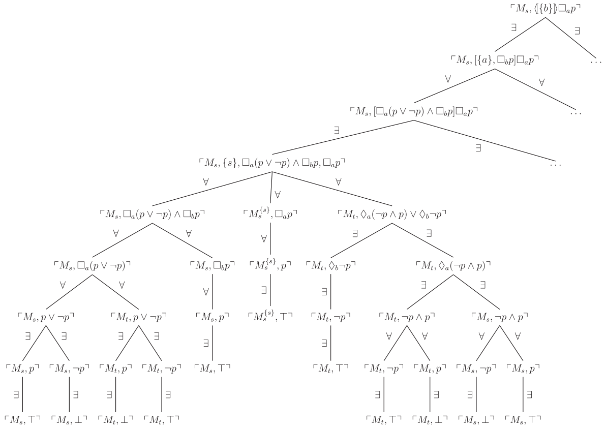
FIGURE A.3. Formula game for \llbracket \{b\} \rrbracket \Box_a p over M_s .
