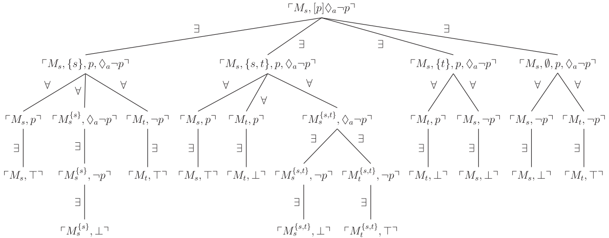
FIGURE A.2. Formula game for [p]◇_a¬p over M_s .
