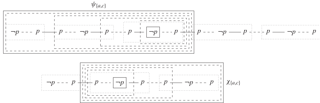
FIGURE 15. An a -model (above) and a b -model (below).
