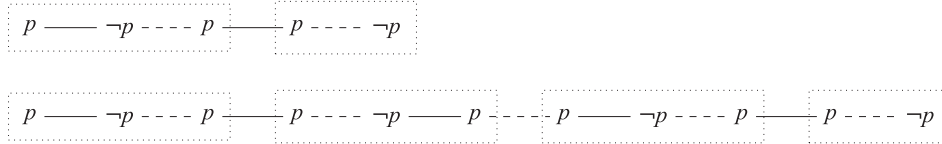
FIGURE 8. [0,4]-Models.
