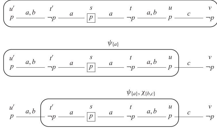
FIGURE 16. Model M_s and an its updates M_s^{\psi_{\{a\}}} and M_s^{\psi_{\{a\}}, \chi_{\{b,c\}}} , with the current model depicted in the rounded rectangles.
