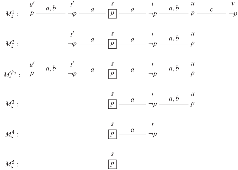
FIGURE 4. Model M_s^1 and various restrictions thereof.
