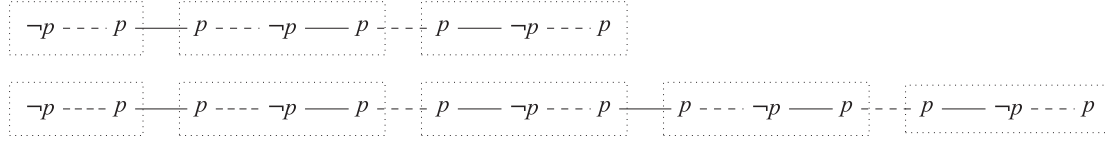
FIGURE 7. [1,2]-Models.
