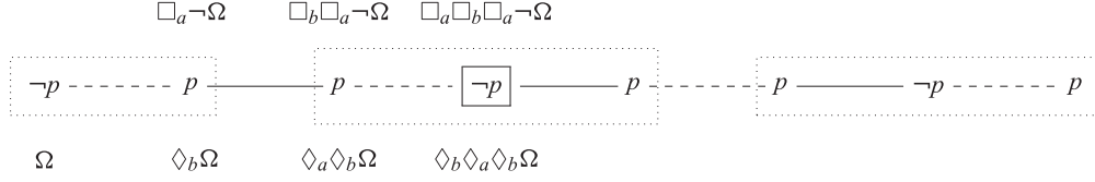
FIGURE 10. Removing states from a model using \Omega .
