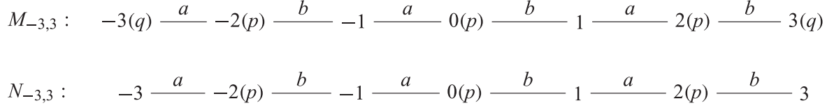
FIGURE 4. The models M_{-3,3} and N_{-3,3} .
