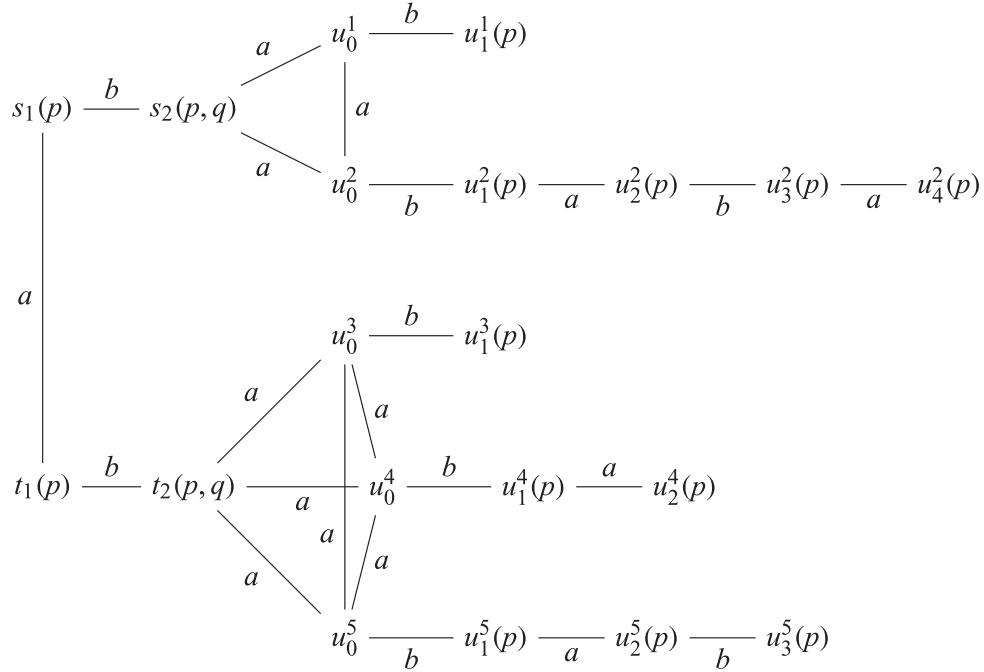
FIGURE 5. Typical model used in the proof that APAL \prec IPAL.
