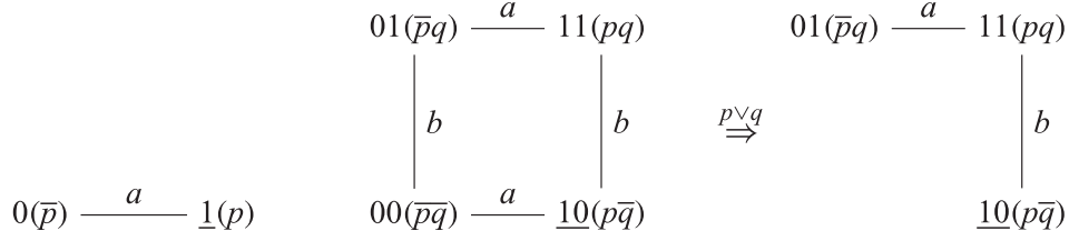
FIGURE 2. Model (N, 1) on the left, (M, 10) in the middle, (M|(p \vee q), 10) on the right.
