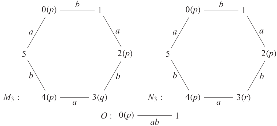
FIGURE 3. The models M_3 and N_3 .
