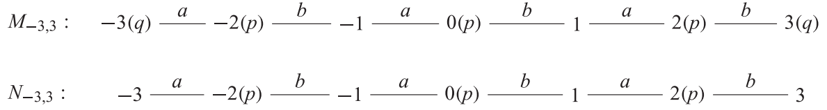
FIGURE 4. The models M_{-3,3} and N_{-3,3} .
