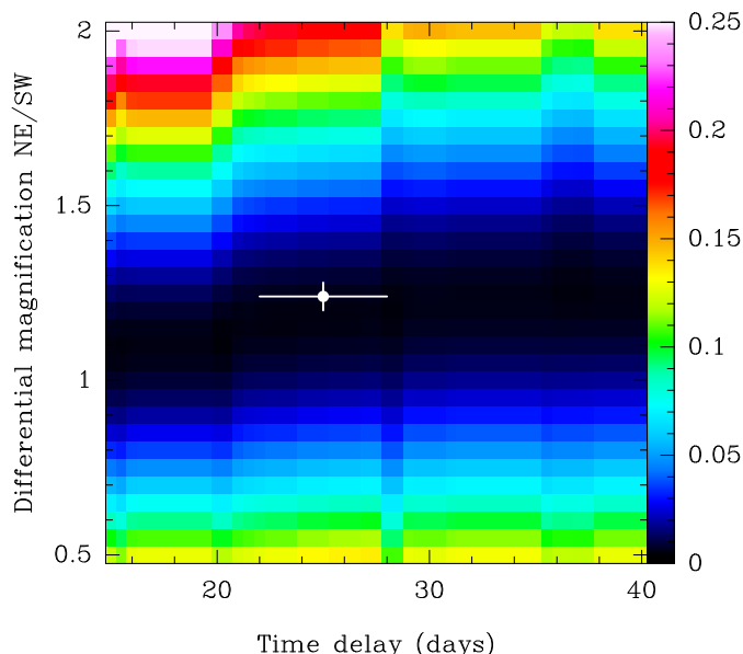
Fig. 3. Measure of randomness using the Von Neumann estimator \mathcal{E}_{\text{VN}} (defined in Eq. 1) as a function of the time delay and differential magnification parameters. The best-fit value obtained from a parametric model of the continuum evolution (Sec. 3.6) is shown by the white mark.
