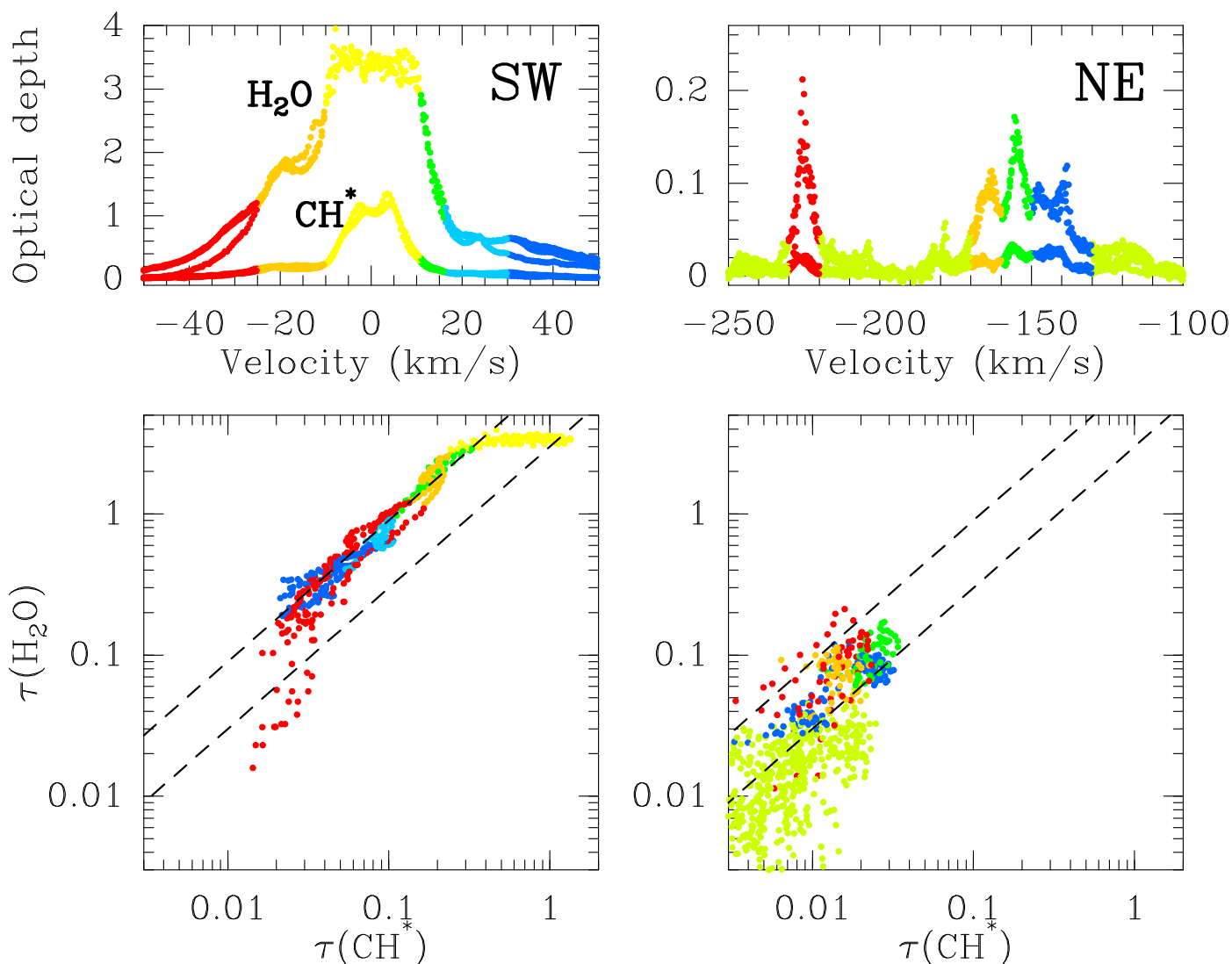
Fig. 18. Correlation between the optical depths of the ortho-H 2 O 1 1,0 – 1 0,1 line and of the deconvolved profile of CH 3/2-1/2 (given for an equivalent hyperfine component with normalized intensity S_{ul} = 1 ) along the SW ( left ) and NE ( right ) lines of sight, respectively. In both lines of sight, we assume a source-covering factor of f_c=1 . The colors encode the velocity intervals shown on the line profiles (top). The dashed lines correspond to opacity ratios \tau(\text{H}_2\text{O})/\tau(\text{CH}^*)=3 and 9, respectively.
