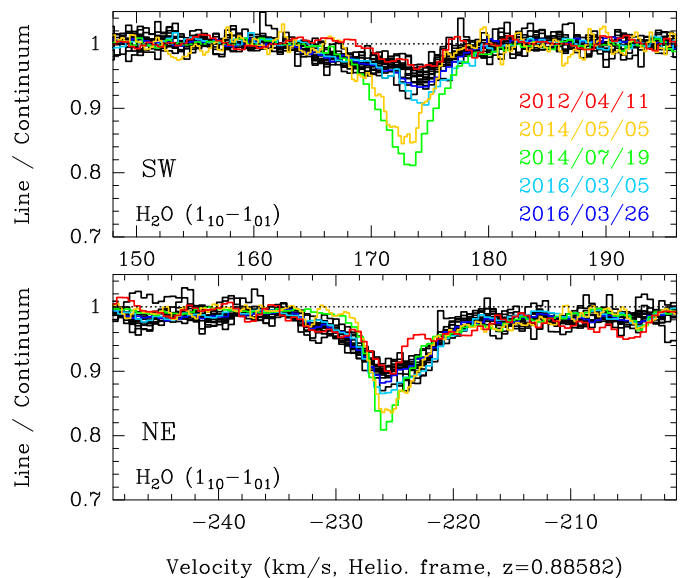
Fig. 7. Zoom onto the variations of the +174 \text{ km s}^{-1} (top) and -225 \text{ km s}^{-1} (bottom) features in the \text{H}_2\text{O} SW and NE spectra, respectively. Same as for Fig. 6; special profiles showing clear deviations are highlighted with the color code given in the upper box.
