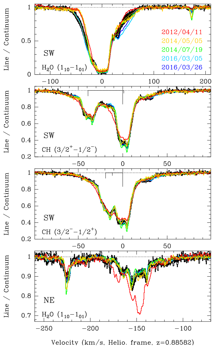
Fig. 6. Overlay of all ALMA spectra of \text{H}_2\text{O} (SW and NE lines of sight) and \text{CH} (SW only) observed toward PKS 1830–211 between 2012 and 2016. Special profiles showing clear deviations are highlighted with the color code given in the upper box.
