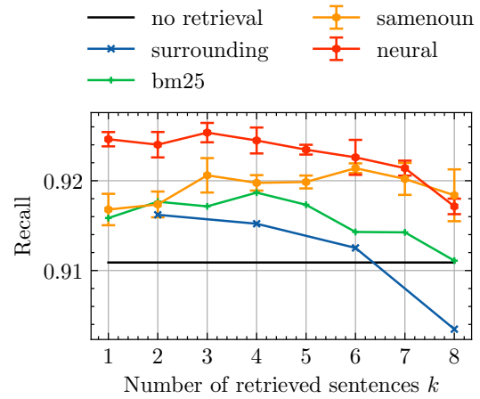
Figure 5: NER Recall using different retrieval methods versus the number of sentences retrieved k .
