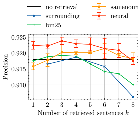
Figure 4: NER Precision using different retrieval methods versus the number of sentences retrieved k .
