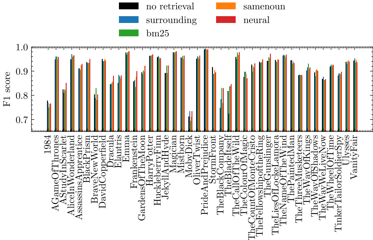
Figure 6: NER F1 Score per book for different retrieval methods, with a number of retrieved sentences k = 1 .
