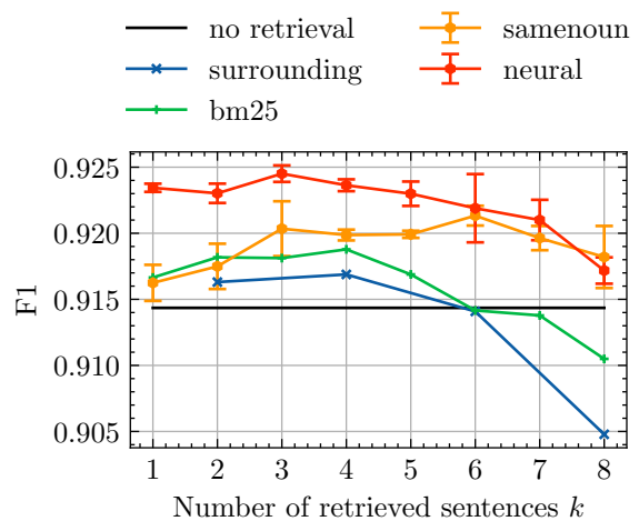
Figure 3: NER F1 score using different retrieval methods versus the number of sentences retrieved k .
