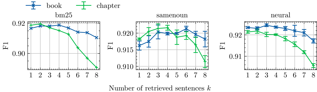
Figure 7: NER performance of different retrieval methods for different context window sizes as a function of the number of retrieved sentences k .
