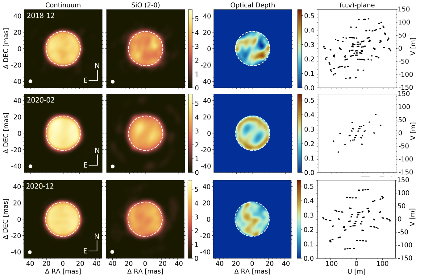
Figure 2. Each rows correspond to a given epoch precised in the top-left corner of the first panel. From left to right: 1) Reconstructed map in the pseudo-continuum, 2) in the SiO (2–0) absorption band (both scaled in Jy/pix with a squared pixel size of 0.78 mas), 3) deduced map of the optical depth for the SiO (2–0), 4) (u,v)-plane coverage of the used measurements. The dashed white circles on the maps enclose intensities higher than 70% of the maximum (42 mas in diameter). The small white disks at the bottom left corners of the reconstructed maps corresponds to an equivalent circular interferometric beam used for the convolution of all the reconstructed images ( \approx 4 mas in diameter). The angular size has been estimated using the Feb. 2020 observations which has the poorest (u,v)-plane coverage among the three epochs.
