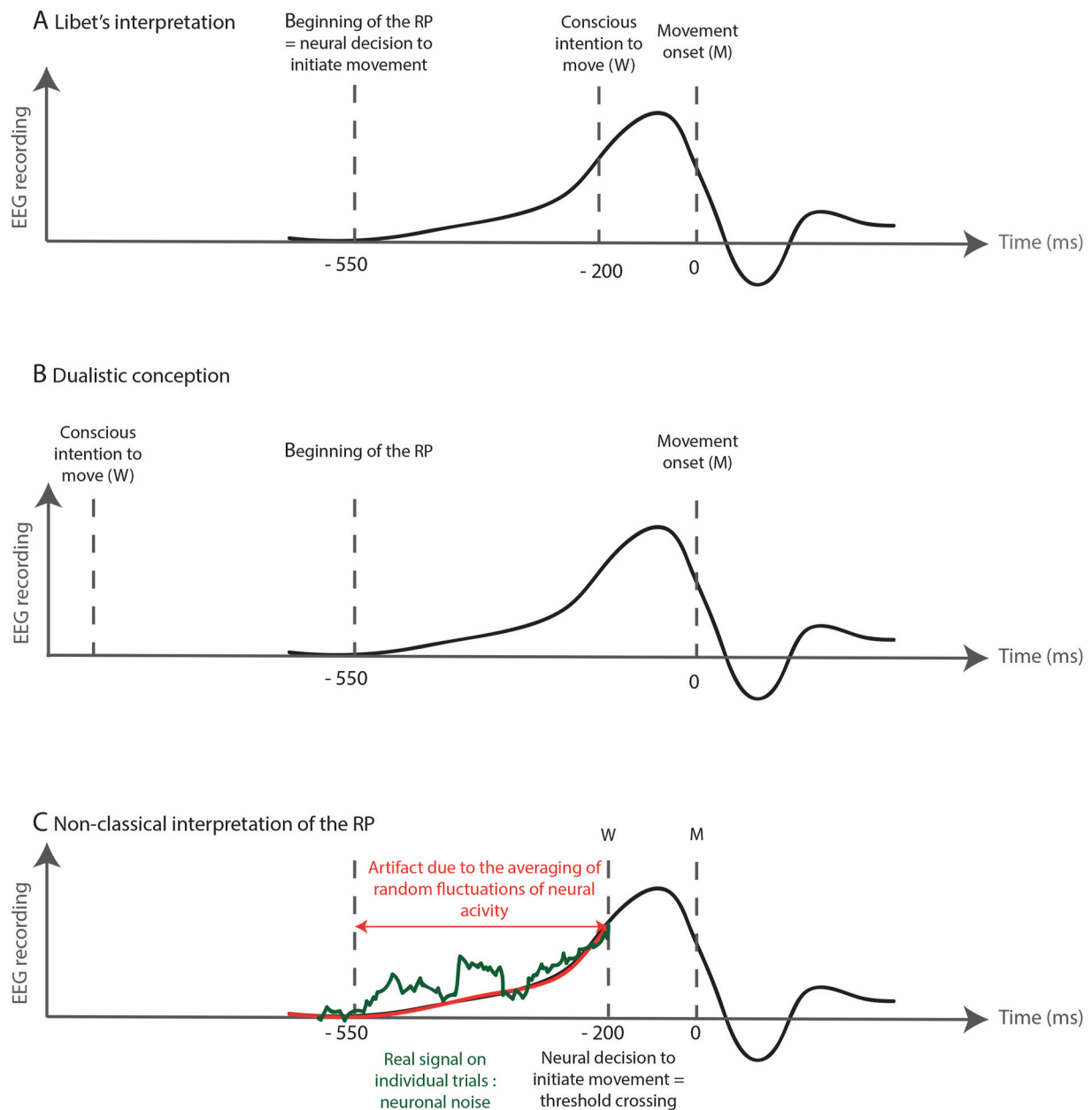
Fig. 4. Different theoretical possible outcomes of Libet's experiments.
