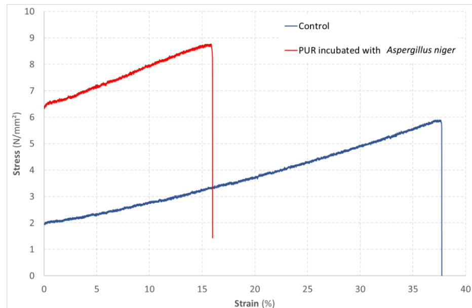
Figure 5. Evolution of the strain of a PUR material as a function of the stress applied in a tensile test. Comparison of an unexposed material (control) with a material exposed to the growth of Aspergillus niger according to method B' of the ISO 846 standard.
