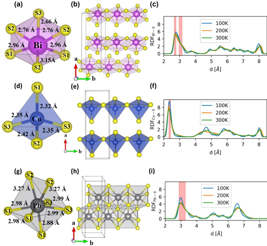
Figure 3. (a) Distorted octahedral coordination of \text{Bi}^{3+} (purple sphere) with sulfur (yellow sphere). (b) One-dimensional [\text{BiS}_4]^- chains directed along the b -axis. (c) Bi-S radial pair distribution function (RDF) computed from the NVT ab initio molecular dynamics trajectory. (d) Distorted tetrahedral coordination of \text{Cu}^+ (blue sphere) with sulfur. (e) Chains of corner-sharing [\text{CuS}_4]^{7-} tetrahedra along the b -axis. (f) Cu-S RDF computed from the NVT ab initio molecular dynamics trajectory. (g) Capped octahedral coordination of \text{Pb}^{2+} (grey sphere) with sulfur. (h) Ribbons, of stoichiometry [\text{PbS}_3]^- , directed along the b -axis. (i) Pb-S RDF computed from the NVT ab initio molecular dynamics trajectory. Legend for the RDF plots: blue, orange and green lines correspond to simulations at 100, 200 and 300 K respectively; the red shaded area highlights the experimental distances.
