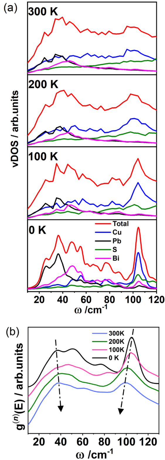
Figure 7. (a) Total (red line) and atom-resolved vDOS of aikinite at different temperatures. Blue, black, green and purple lines correspond to \text{Cu}^+ , \text{Pb}^{2+} , \text{S}^{2-} and \text{Bi}^{3+} ions respectively. The vDOS at 0 K was computed by DFT, and those between 100 and 300 K by AIMD. (b) Neutron-weighted total calculated vDOS convolved with the LET instrumental resolution function, as a function of temperature. Arrows indicate shifts in peak positions.
