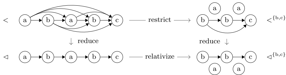
Fig. 1. Piecewise, local, and tier-based factors [18].
