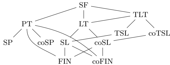
Fig. 2. A hierarchy by subclass of subregular classes.
