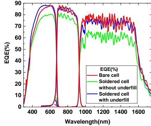
Fig. 4. EQE measurements of bare hexagonal solar cells (red), soldered hexagonal solar cell without underfill (green) and soldered hexagonal solar cell with underfill (blue).
