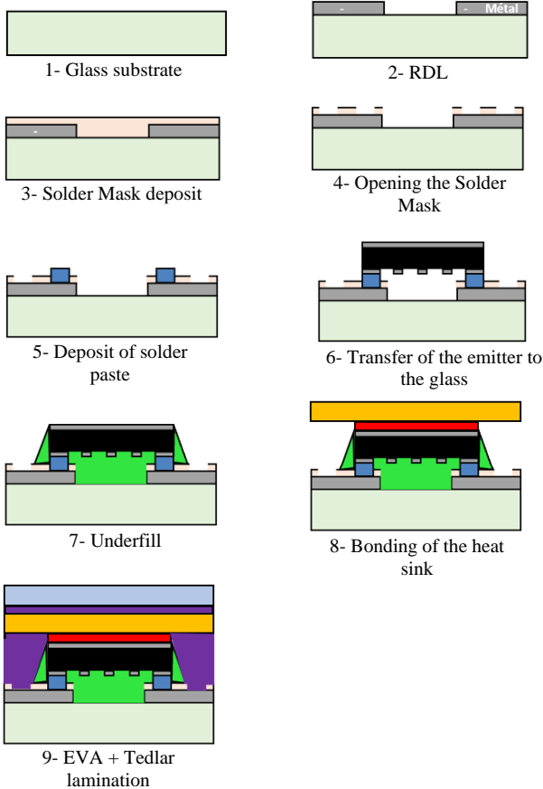
Fig. 1. Process flow of solar cell assembly on glass substrate.
