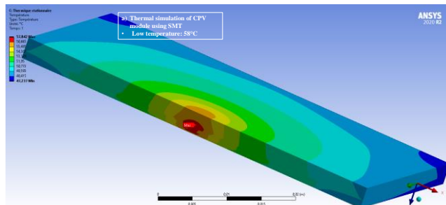
Fig. 10-b. Finite element simulation of CPV module using SMT showing 58°C.
