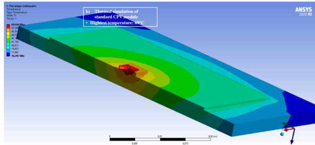
Fig. 10-a. Finite element simulation of standard CPV module showing 69°C.
