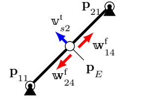
(c) Top view of an RRR mechanism in a singular configuration
