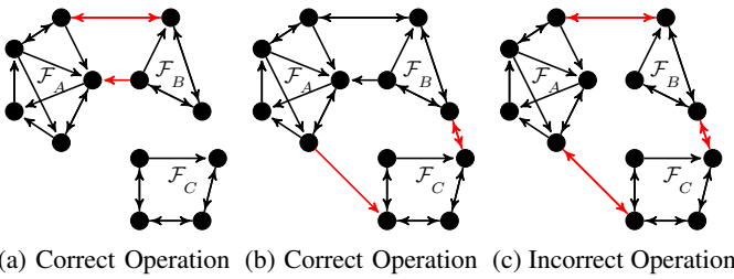
(a) Correct Operation (b) Correct Operation (c) Incorrect Operation Fig. 12: Synthesis of a formation \mathcal{F} with known singularities, from sub-formations \mathcal{F}_A , \mathcal{F}_B , and \mathcal{F}_C . The red edges are edges which are added to join previously separate subformations at a given step in the procedure.
