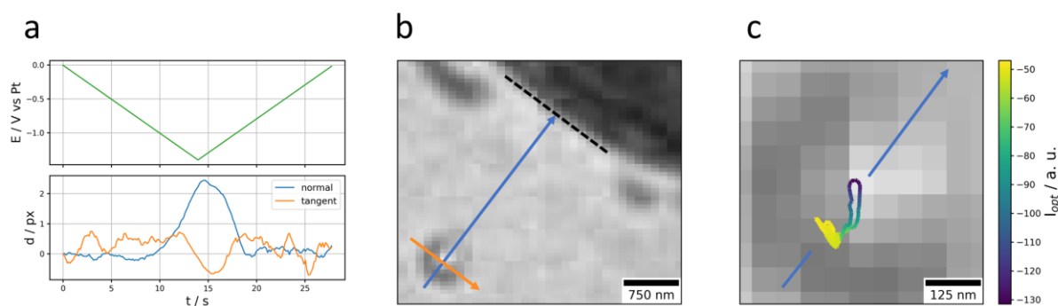
Figure 5: Pinning of the nanodroplet. a Evolution of the applied potential (top, green) and of the displacement (with respect to its initial position) along the normal and tangential direction of the Pt NP discussed in Figure 1 (bottom) over time. The directions are defined in b compared to the reservoir's contact line passing through the NP's initial centre of mass. c Trajectory of the Pt NP with a colour scale conveying its optical intensity.
