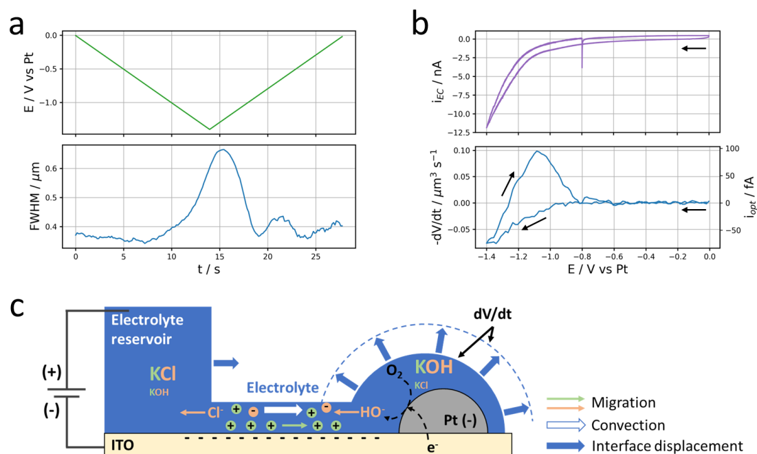
Figure 4: Local current. a Evolution of the applied potential at the ITO electrode (top, green) and the FWHM of the Pt NP discussed in Figure 1 (bottom, blue) over time. b Electrochemical (top, purple) and optical CV (bottom, blue) in terms of current and volumetric flow rate. c Schematic description of the electrokinetic transport through the thin electrolyte film and nanodroplet volume variation ( dV/dt ) induced by electrolysis at the Pt NP. Migration of ions corresponds to electrophoretic, EP, contribution and convection to electro-osmotic, EO, contribution. The volume variation of the nanodroplet corresponds to difference between the volume of the plain hemisphere and that delimited by the dashed line.
