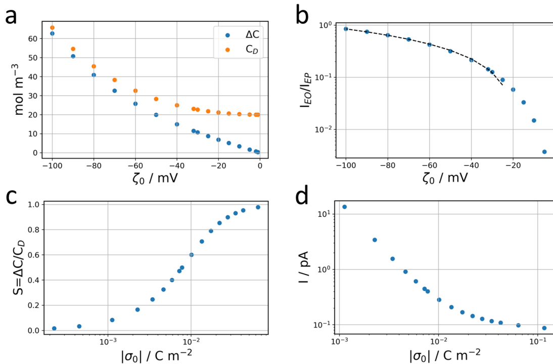
Figure 7: Theoretical framework. a Average concentration difference \Delta C and Donnan concentration C_D in the nanochannel as a function of the zeta potential of the ITO surface for a 10 mM KCl bulk electrolyte. b Ratio between the electro-osmotic, EO, and electrophoretic, EP, contributions to the ionic current across the channel as a function of the zeta potential of the ITO surface. c Selectivity of the nanochannel as a function of the surface charge held by the ITO. d Total ionic current across the nanochannel evaluated for a fixed value of I_{EO} = 50 \text{ fA} for different values of the surface charge (equiv. zeta potential) held by the ITO.
