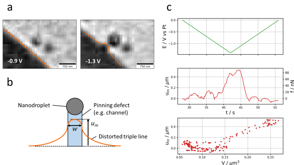
Figure 6: Pinning of the reservoir's contact line. a Optical images of another Pt NP at different potentials showing the deformation of the reservoir's contact triple line (orange dashed line) towards the Pt NP and revealing the actual channel between the electrolyte reservoir and the Pt NP at very negative potentials. b Schematic description of the deformation of the contact triple line by a band-shaped defect of high surface energy from which the defect apparent width w and triple line elongation u_m (pinning force) is estimated. The scheme also shows that the triple line is not pinched by the nanodroplet but by the nanochannel. c Evolution of the applied potential (top, green) and of elongation or pinning force (middle, red) over time. The bottom figure shows the correlation between the triple line elongation and the volume changes of the nearby NP.
