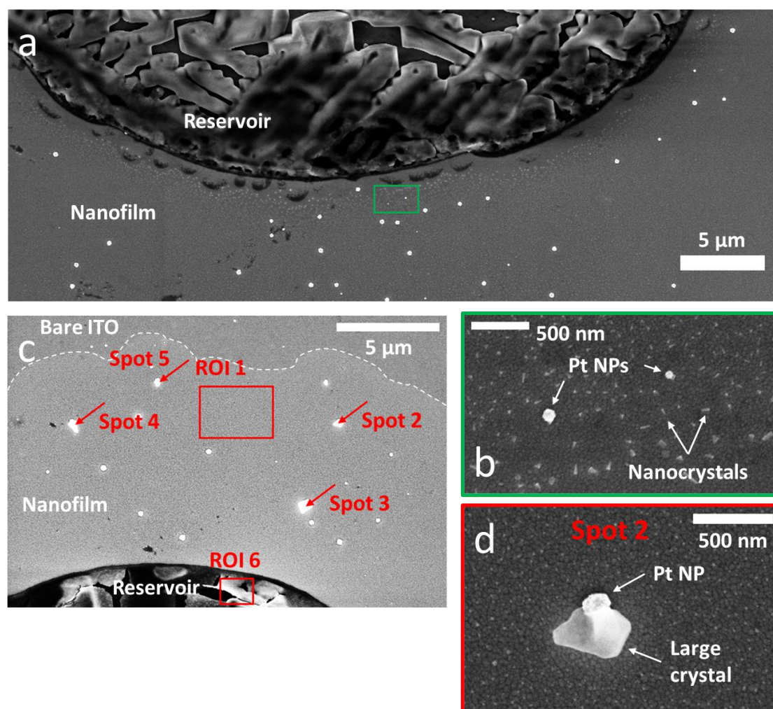
Figure 3: SEM. a SEM image acquired post-mortem in the same location as Figure 1b. b High-magnification SEM of the ROI highlighted in green in a showing two Pt NPs surrounded by multitude of nanocrystals forming all around the electrolyte reservoir. c SEM image of another part of the sample showing the expansion of the nanofilm (brighter region delimited by the dotted line). This region, not monitored optically, shows larger crystals formed around some Pt NPs. The red rectangles and arrows highlight the regions and spots analysed by EDX (see Table 1). d High-magnification SEM image of the Pt NP and crystal called “spot 2” in c .
