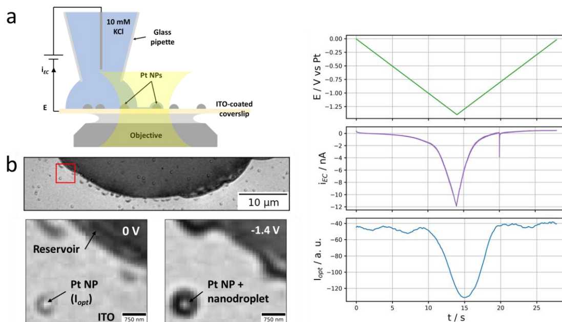
Figure 1: Setup and first observations. a Scheme of the experimental configuration. b Widefield optical image of the electrolyte reservoir and peripheral Pt NPs (top) and zoom over the region of interest, ROI, highlighted in red at 0 V and -1.4 V vs Pt (bottom). In the zoomed regions are detailed the reservoir, NP and nanodroplet, the optical intensity is evaluated over the NP region (see Materials and Methods). c Evolution of the applied potential (top, green), the measured electrochemical current (middle, purple) and the optical intensity of the Pt NP highlighted in b (bottom, blue) over time.
