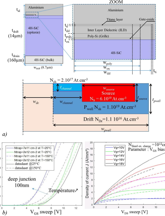
Fig. 1 a) Parametric basis of 1.2kV-80mΩ half-cell gate-planar 4H-SiC MOSFET 2D model and b) static results.
