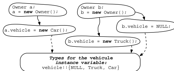
Figure 2. Type flow analysis for instance variable vehicle from class OWNER . Order of statements is not relevant and the result which is \{\text{NULL}, \text{TRUCK}, \text{CAR}\} , is for all instances of the class OWNER .
