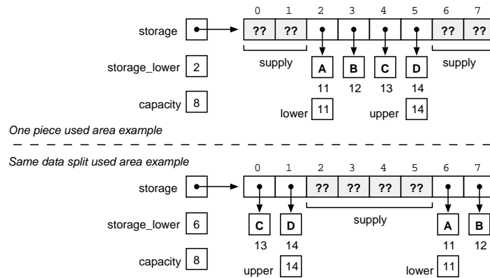
Figure 4. Implementation of a RING_ARRAY with 5 variables. The user's visible range is [lower, upper] . The storage_lower internal variable is the corresponding index of element at lower index inside storage . Because the used area unfolds circularly starting at any possible storage_lower , there are many possibilities.
