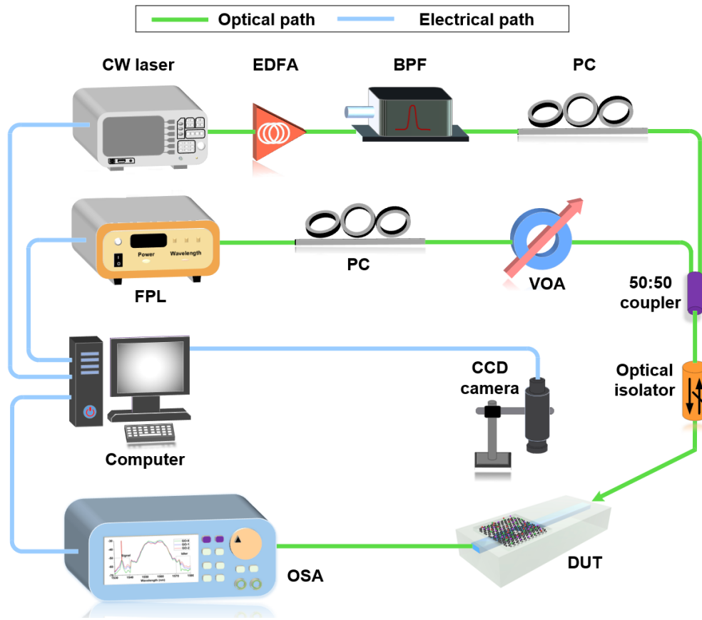
Figure 3. Experimental setup for OPA experiments. CW laser: continuous-wave laser. FPL: fiber pulsed laser. PC: polarization controller. EDFA: Erbium doped fiber amplifier. VOA: variable optical attenuator. OPM: optical power meter. DUT: device under test. CCD: charged-coupled device. OSA: optical spectrum analyzer.
