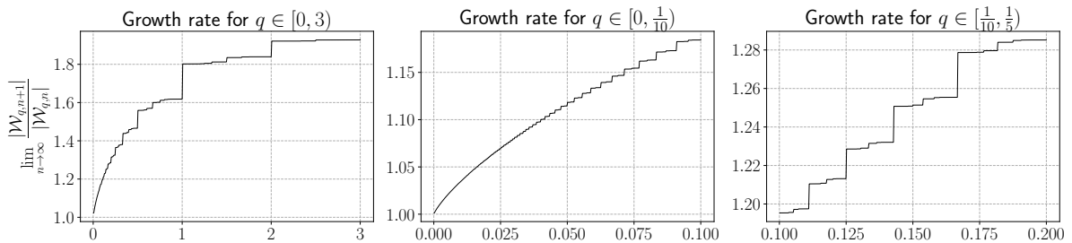
Figure 2: \lim_{n \rightarrow \infty} |\mathcal{W}_{q,n+1}|/|\mathcal{W}_{q,n}| as a function of q in three different intervals. This function is jump discontinuous at every positive rational point.
